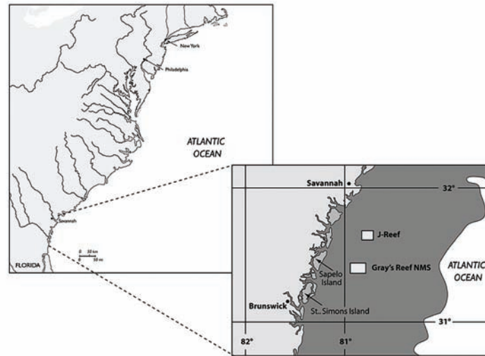
Figure 1. The Georgia Bight highlighting the study area of Gray's Reef National Marine Sanctuary and J-Reef.
