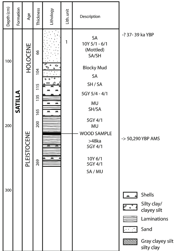
Figure 3. Vibracore from the J-Reef paleochannel’s estuarine-fluvial depositional regime of laminated sand-mud and clay Satilla Formation strata with a Unit 1 sand cover. Munsell colors and absolute date ranges are shown.
