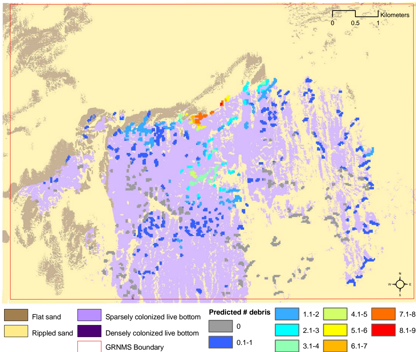
Figure 3.11. Interpolated debris density (per 100 m 2 ) in GRNMS from ordinary kriging.
