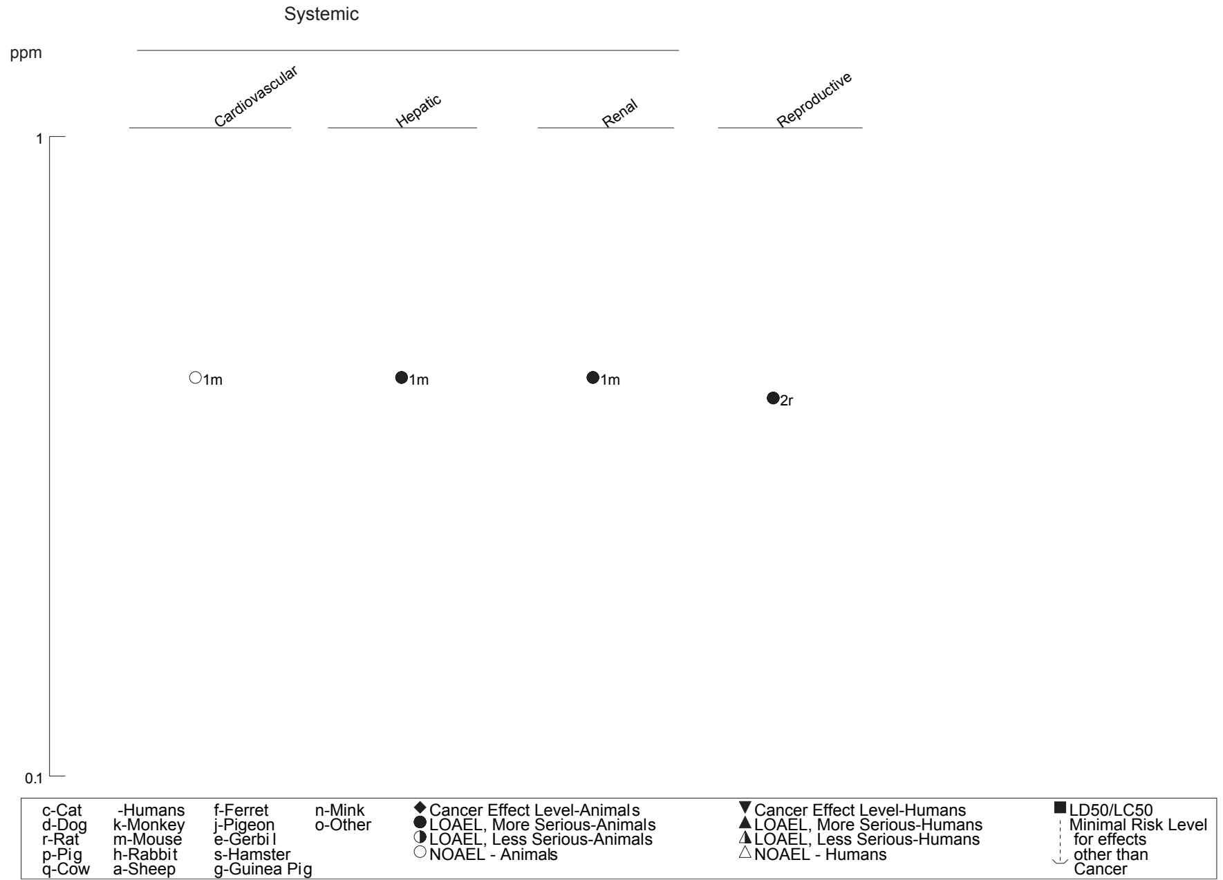
Figure 3-1 Levels of Significant Exposure to Tributyltins - Inhalation Acute (≤14 days)
