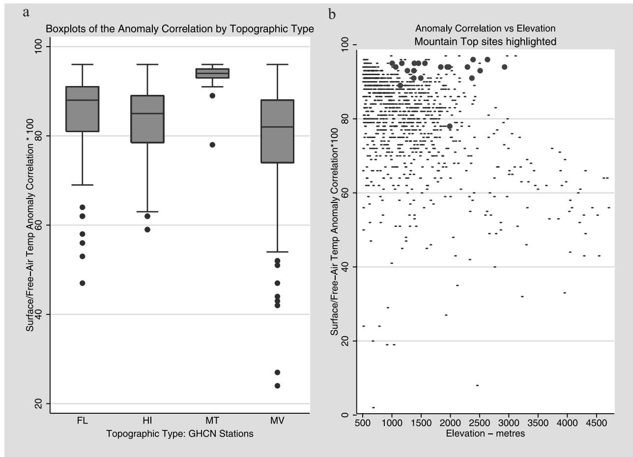
Figure 3. (a) Analysis of variance of the surface/free-air temperature anomaly correlation by topographic class for GHCN stations. Correlations are multiplied by 100. Topographic types are FL, flat; HI, hilly; MT, mountaintop; and MV, mountain valley. (b) Anomaly correlation (multiplied by 100) versus station elevation for all sites (GHCN and CRU). Mountaintop sites are highlighted as large circles.
