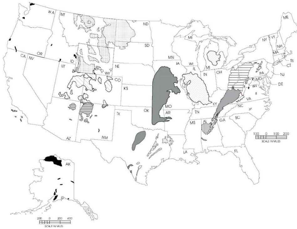
Figure 6. Coal Market Module (CMM) Regional Map
