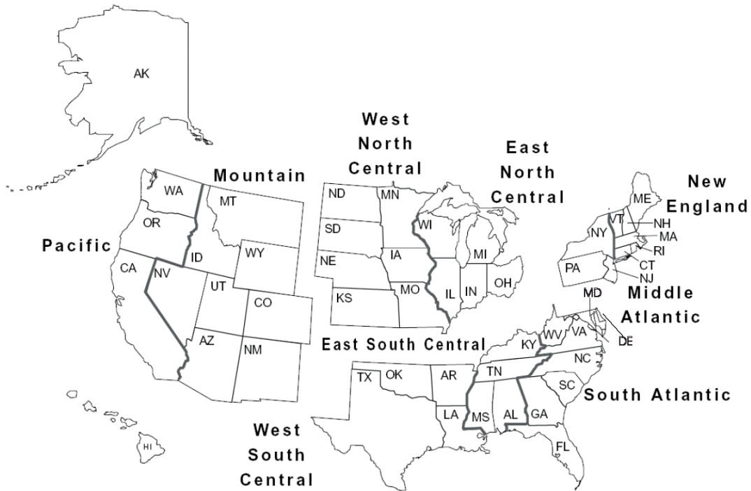
Figure 1. United States Census Divisions
