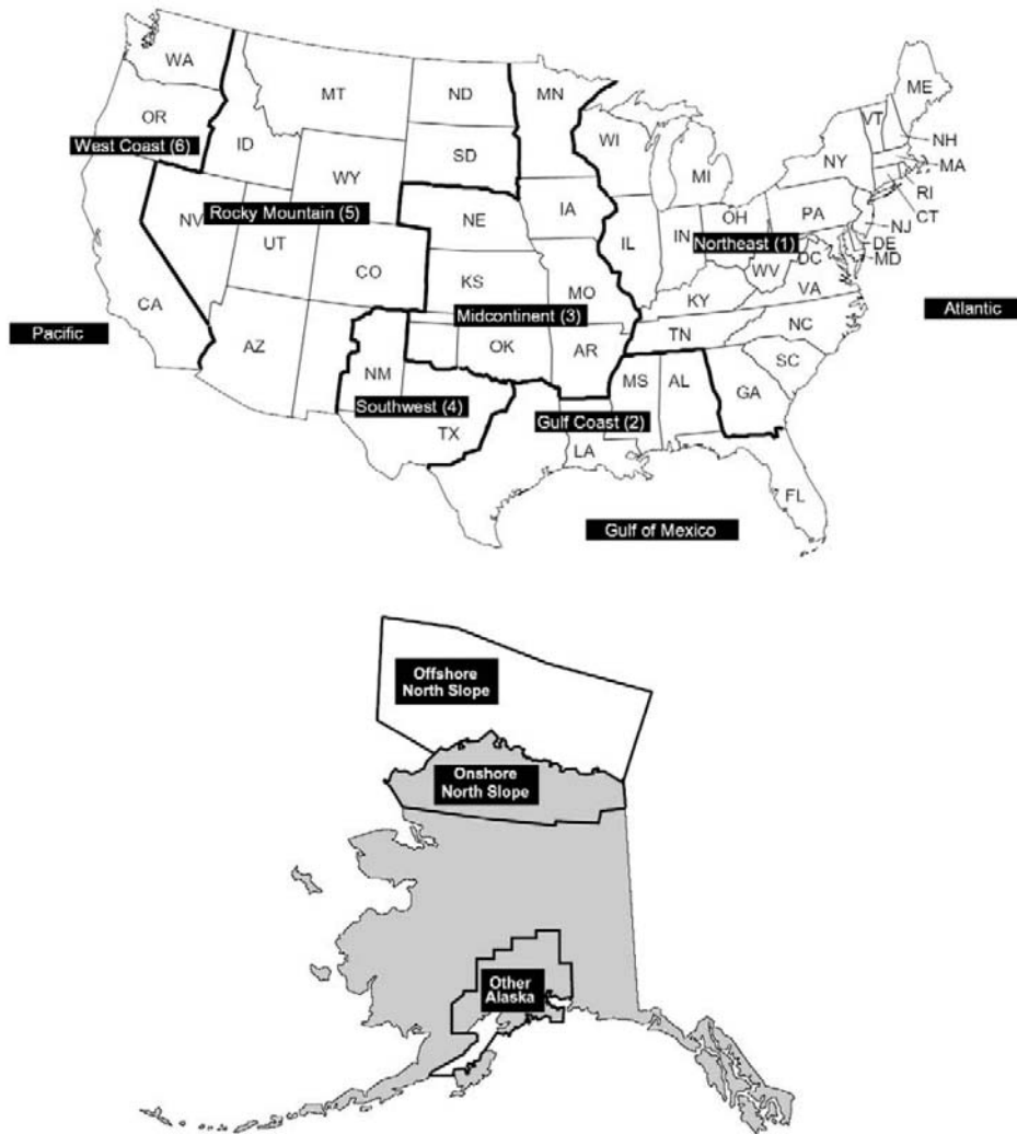
Figure 4. Oil and Gas Supply Model Regions
