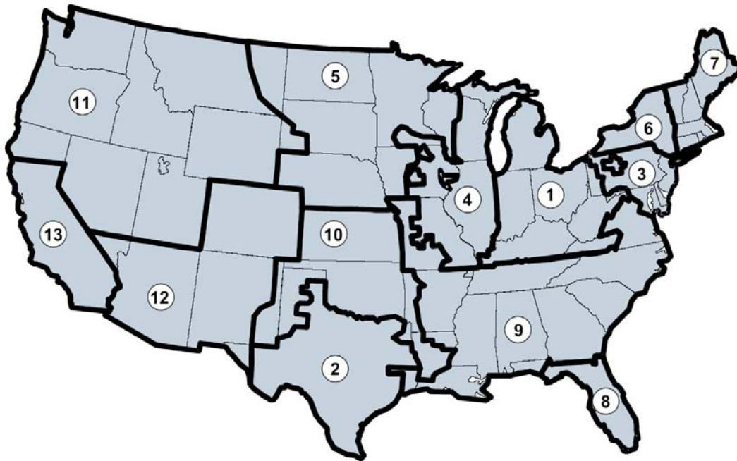
Figure 2. Electricity Market Module (EMM) Regions
