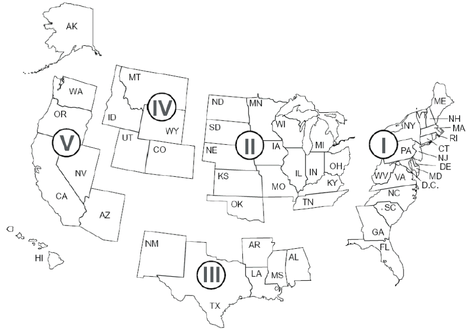
Figure 3. Petroleum Administration for Defense Districts
