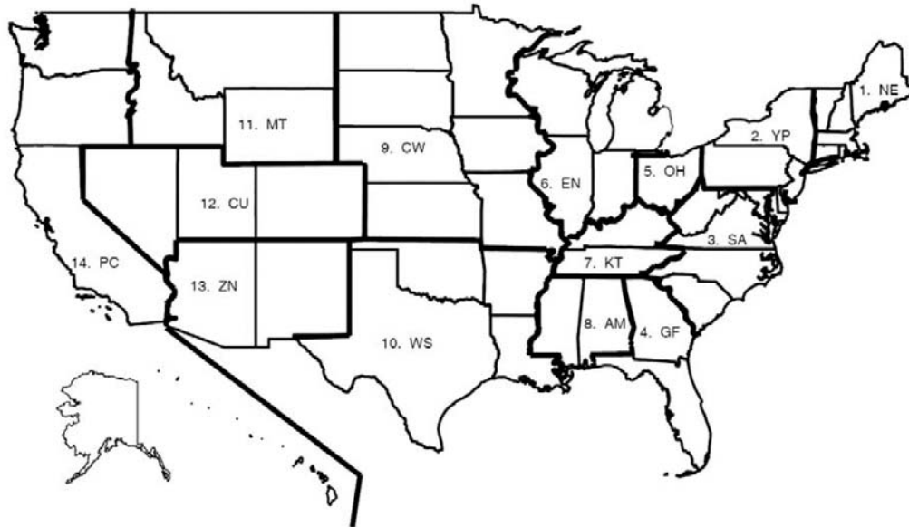
Figure 7. Coal Demand Regions
