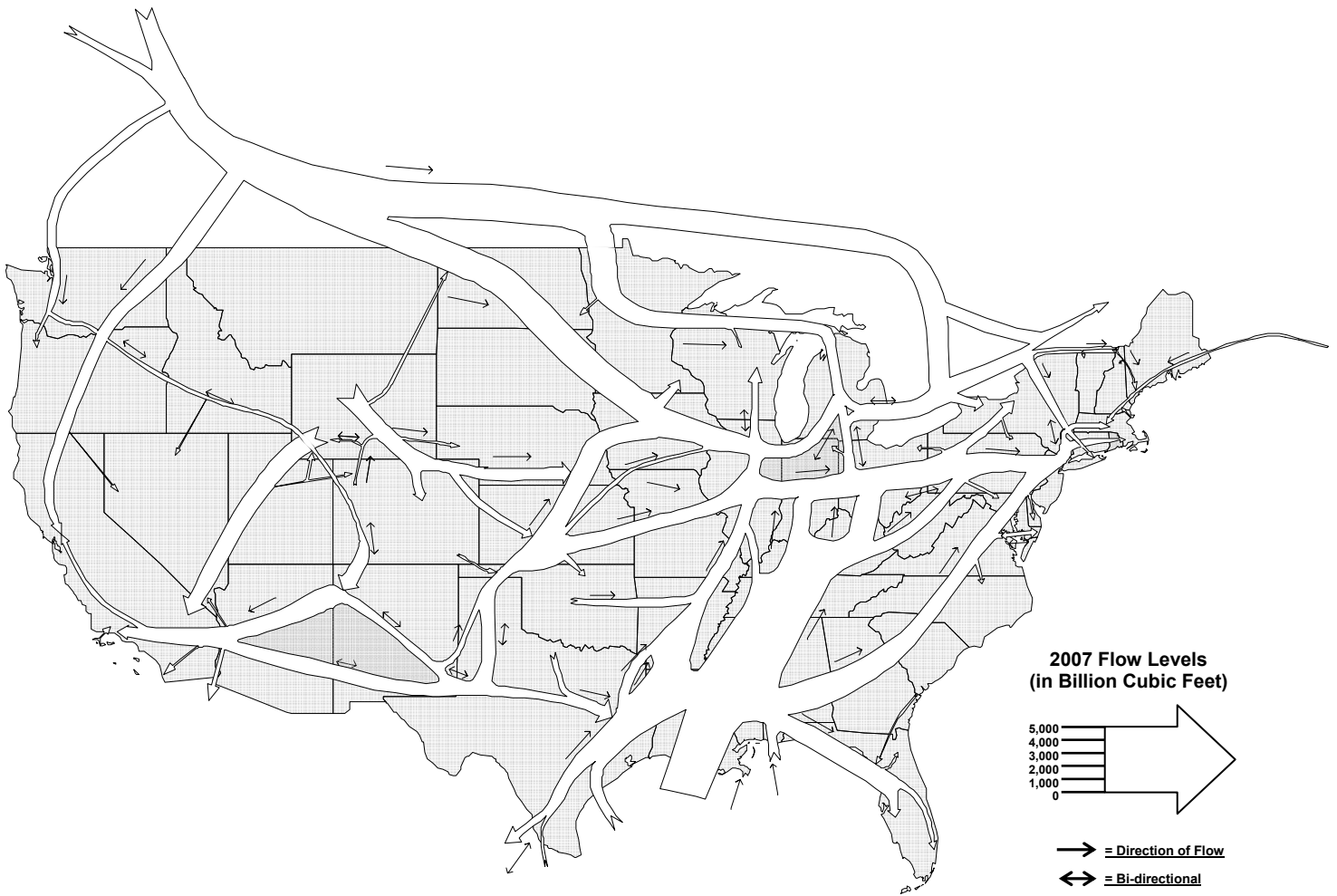
Figure 12. Principal Interstate Natural Gas Flow Summary, 2007
