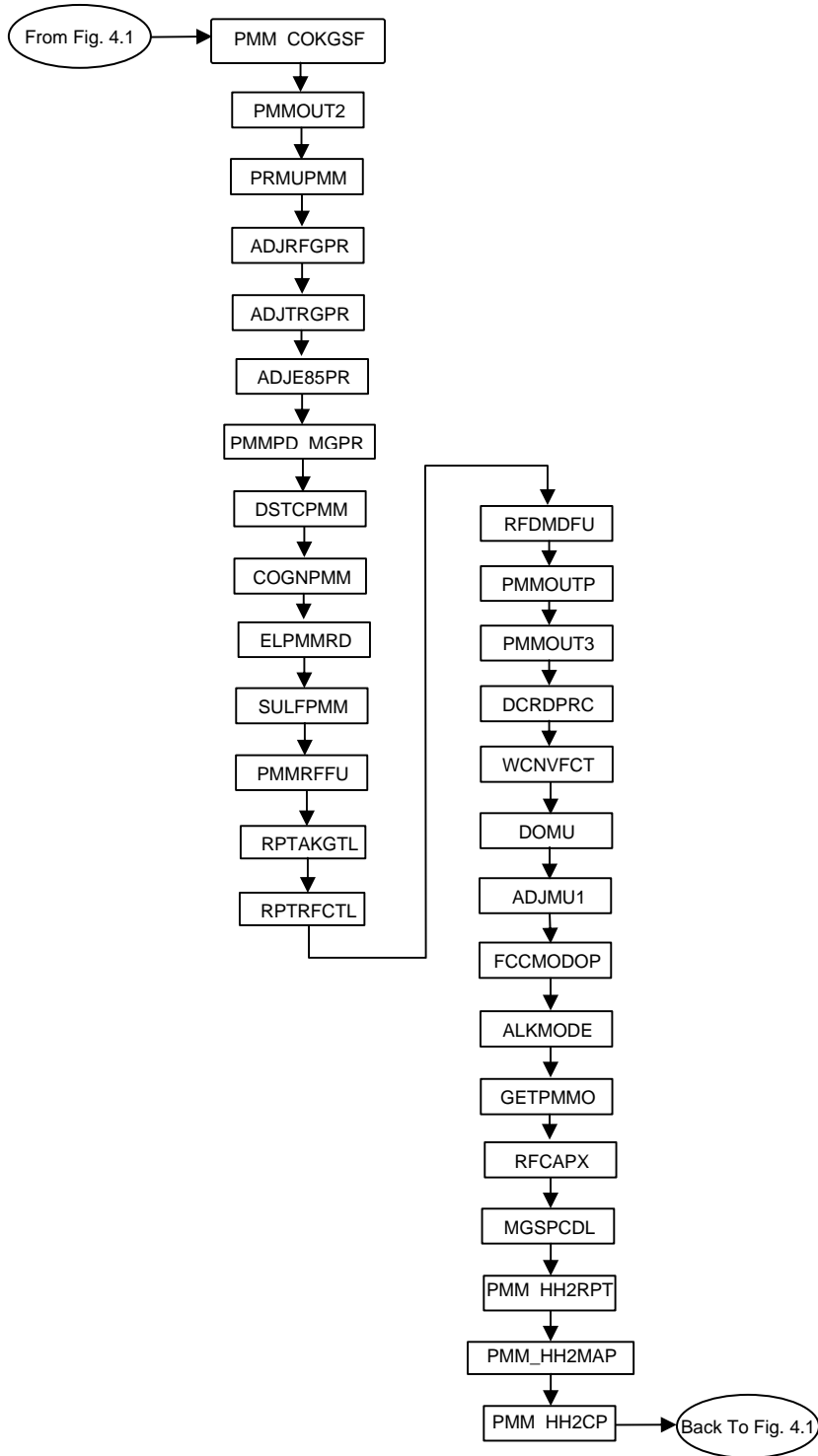
Figure 4.3 Matrix Postprocessing Subroutines
