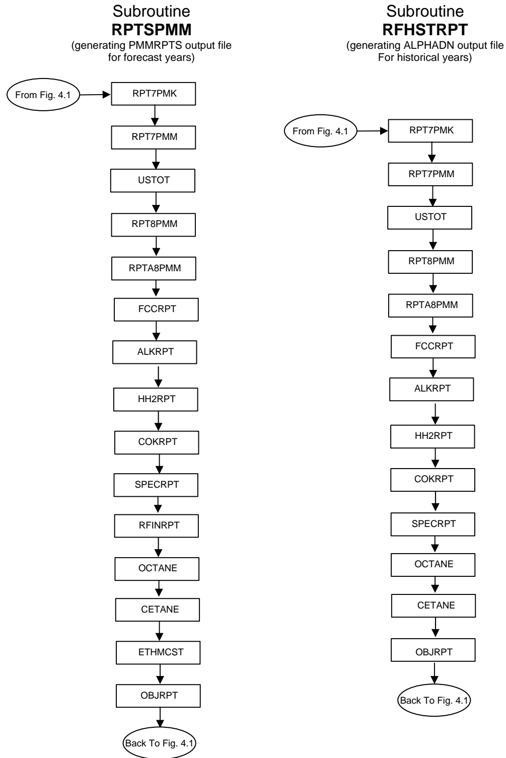
Figure 4.5 Report Subroutines
