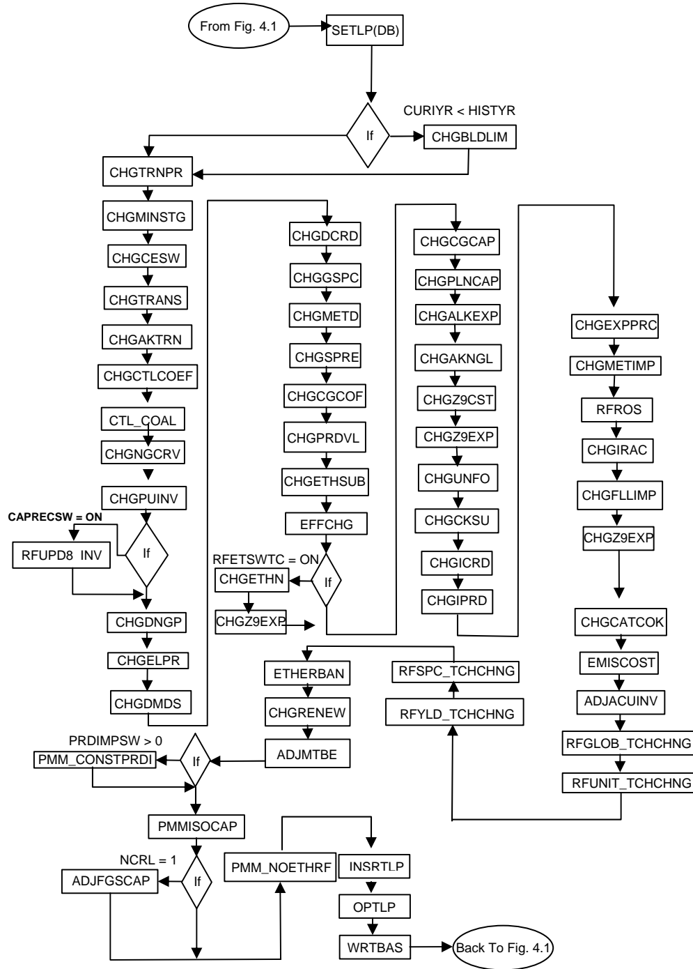
Figure 4.4 Capacity Expansion Subroutines (XPMMLP)
