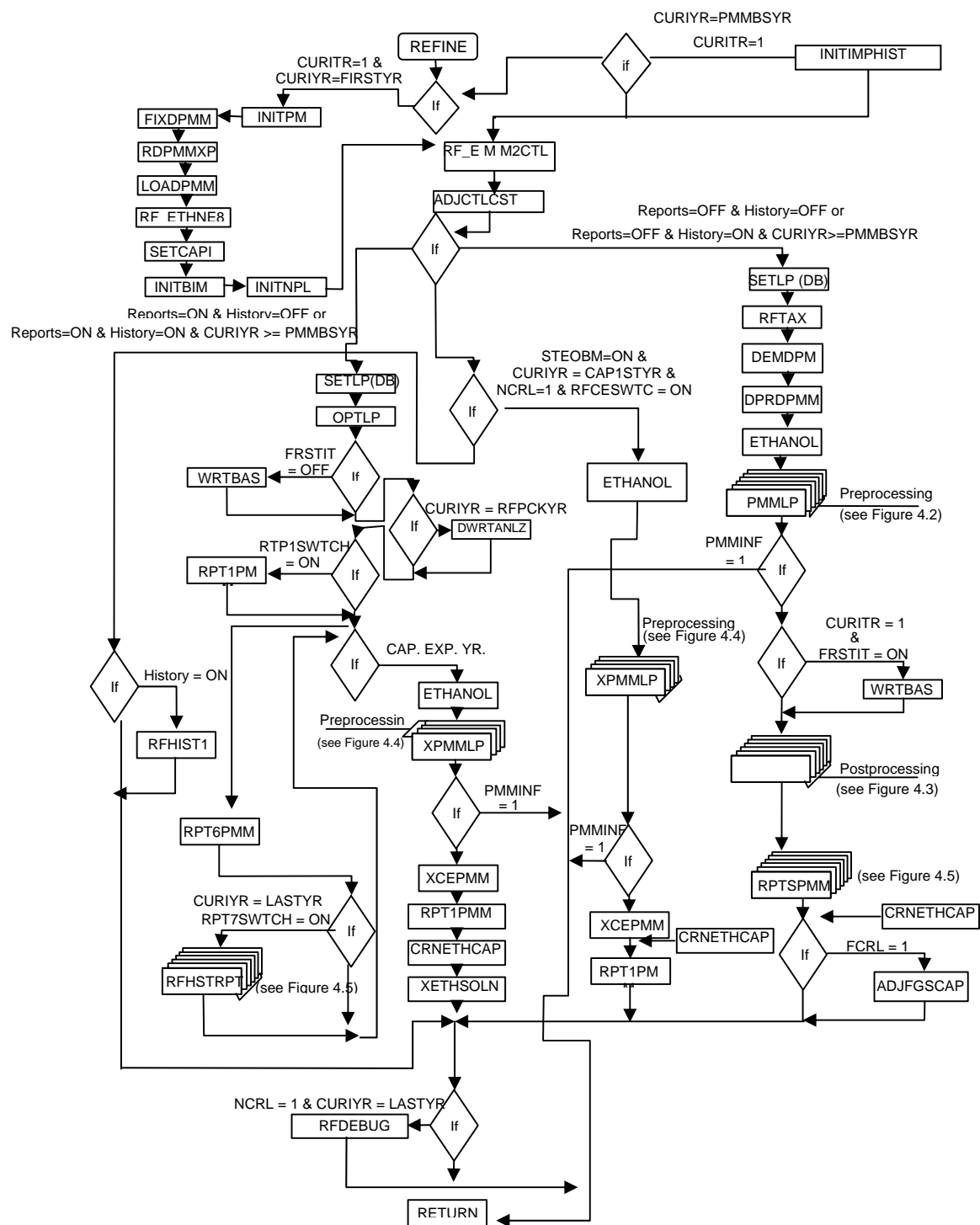
Figure 4.1 PMM Flow Diagram
