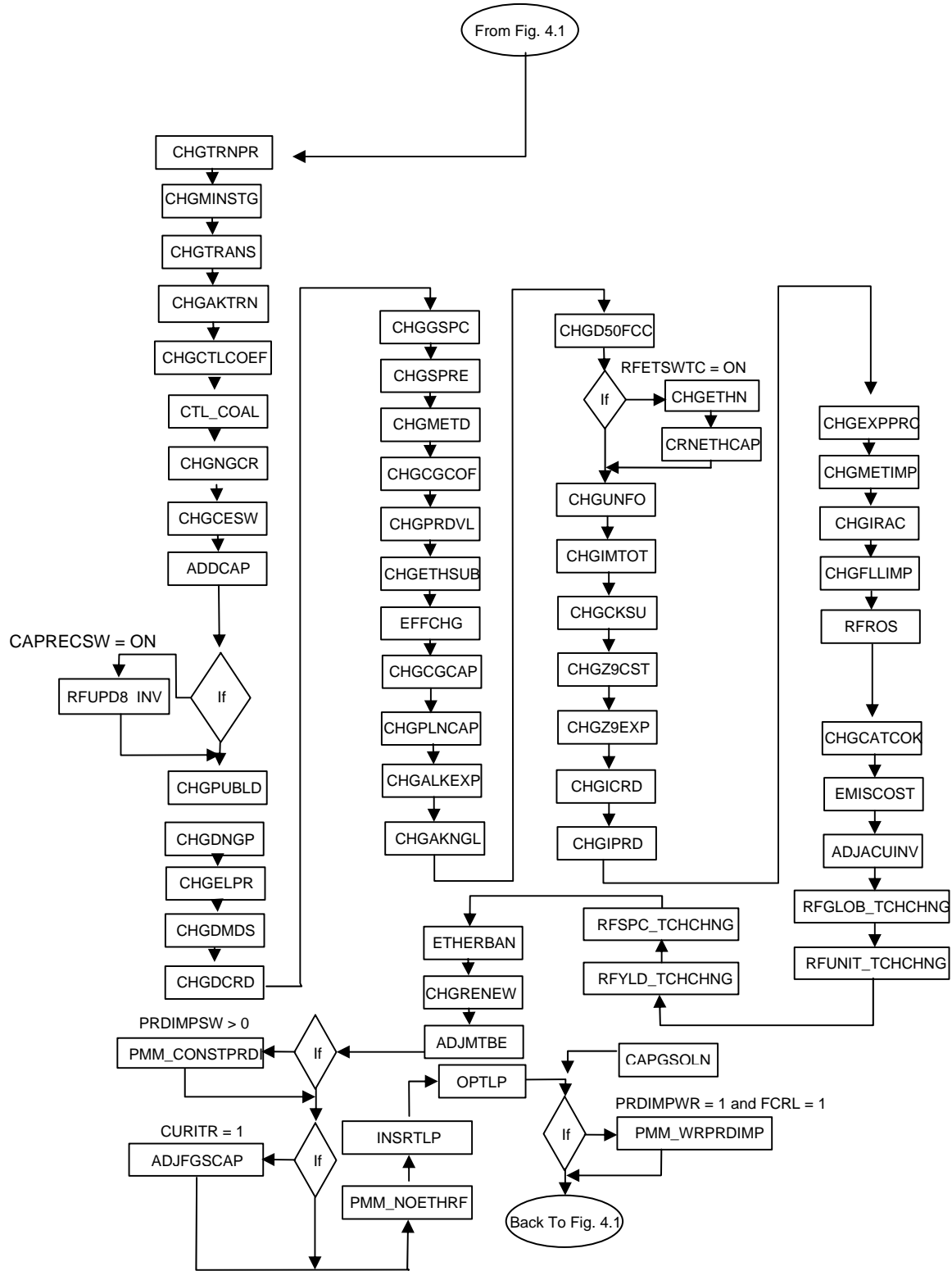
Figure 4.2 Matrix Preprocessing Subroutines (PMMLP)
