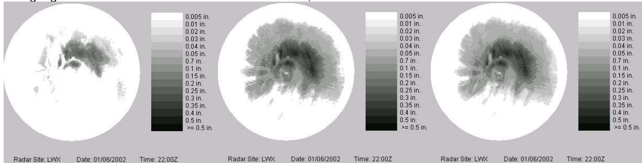
Figure 1. One-hour DPA rainfall from NOFIX (left), SFIX (middle), and EFIX (right) for a stratiform precipitation event (2100-2200 UTC 1/6/2002) 12 hours after the start of the event at KLWX.
