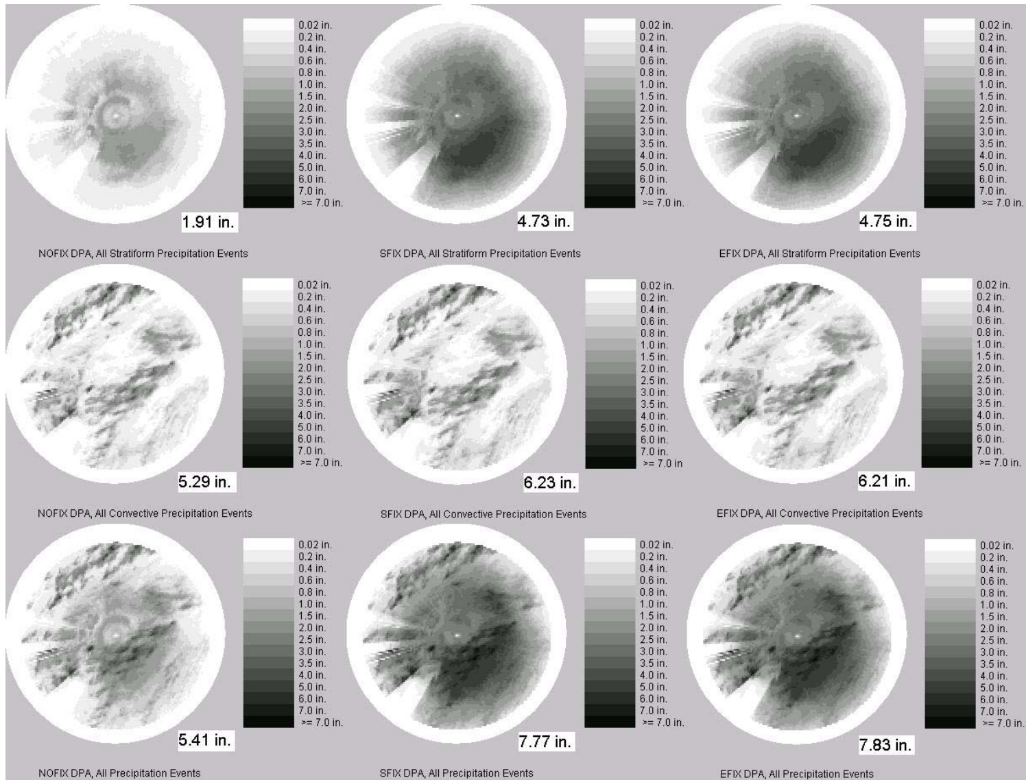
Figure 3. Total rainfall amounts of all the stratiform precipitation events (top), all the convective precipitation events (middle), and all the precipitation events (bottom) from NOFIX DPA (left), SFIX DPA (middle), and EFIX DPA (right). The maximum value is shown in the lower right corner.
