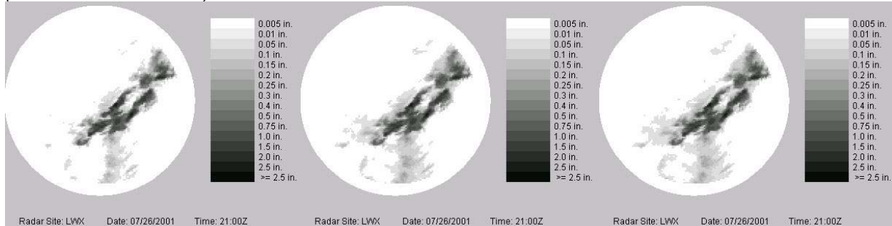
Figure 2. Same as Fig. 1 but for a convective precipitation event at KLWX (2000-2100 UTC 7/26/2001)
