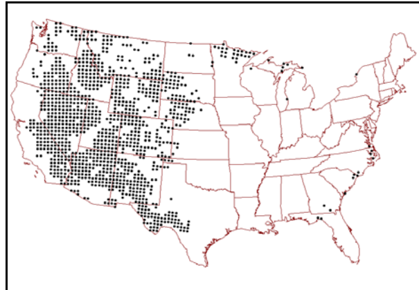
Figure 2. Grid points not used in the AVN MOS severe thunderstorm development.
