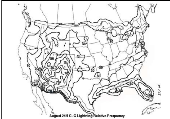
Figure 1. The monthly 24-h (ending at 1200 UTC) cloud-to-ground lightning relative frequency for August.
