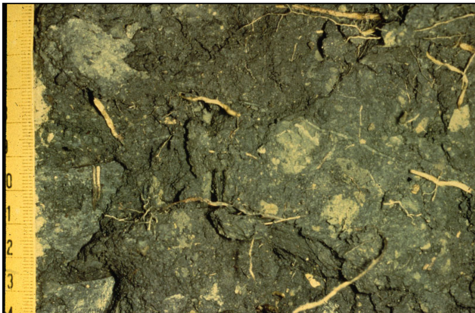
Figure 19. Redox depletions (lighter colored areas) scattered within the darker matrix.
