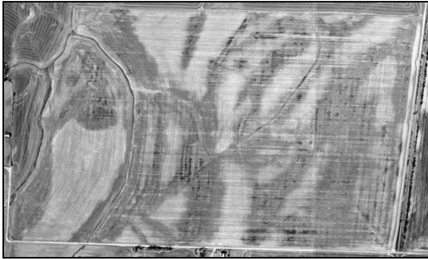
Figure 43. Aerial photograph of an agricultural field with saturated soils indicated by darker colors.
