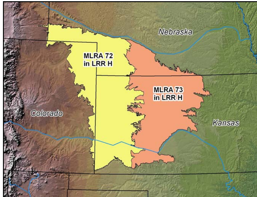
Figure 21. Location of MLRAs 72 and 73 in LRR H.
