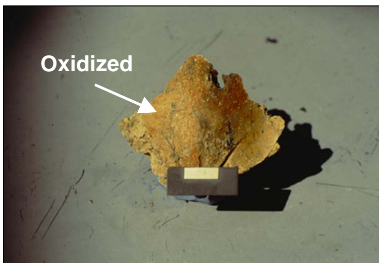
Figure 48. Soil in Figure 47 after exposure to the air and oxidation has occurred.
