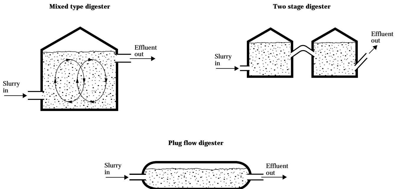
Figure 10-46 Typical anaerobic digester types
