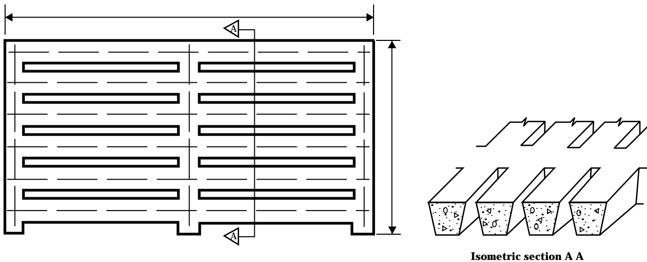
Figure 10-11 Concrete gang slats
