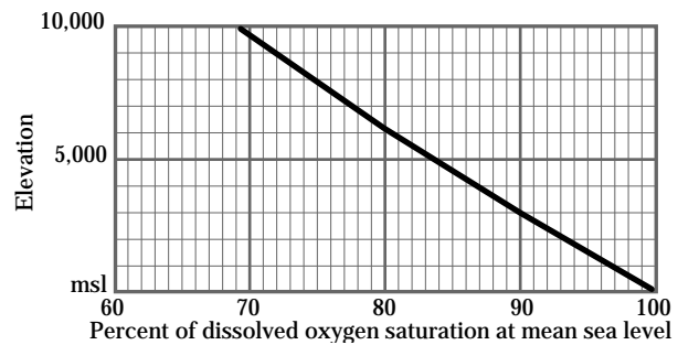
Figure 10-27 Relation of dissolved oxygen saturation to elevation above mean sea level
