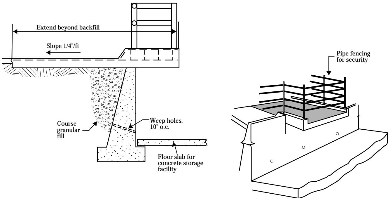
Figure 10-43 Push-off ramp
