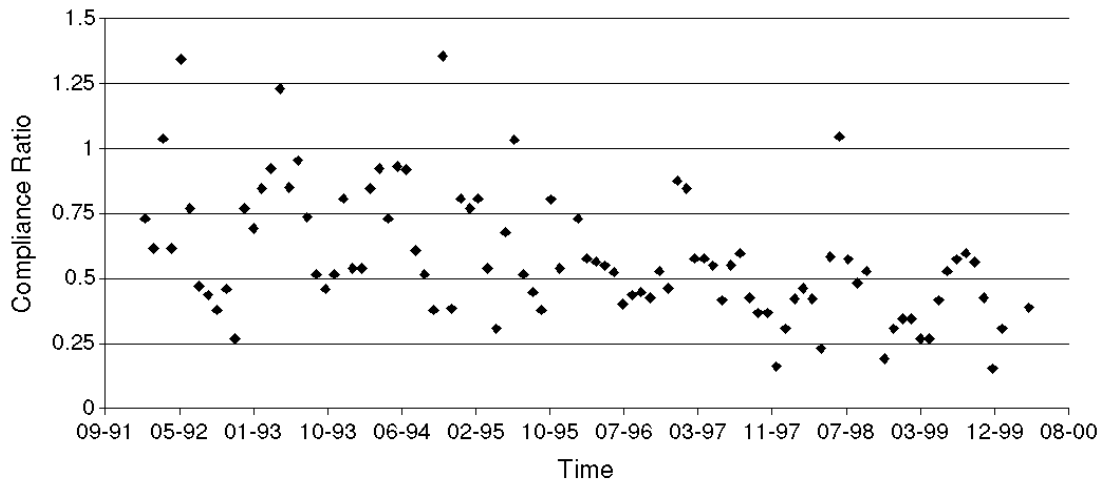
Figure 6 MD0021610: Frederick City WWTP
