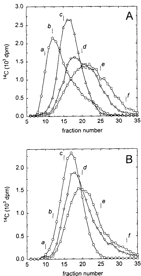
Fig. 2. (A) GPC analyses of phenolic synthetic [ ^{14}\text{C} ]lignin after 6 h of treatment (V) and after 24 h of treatment (£) with laccase/HOBT. A 24-h control reaction that lacked laccase had no effect on the lignin ( \Delta ), whereas a 24-h control reaction that lacked HOBT (O) polymerized it. (B) GPC analyses of nonphenolic (permethylated) synthetic [ ^{14}\text{C} ]lignin after 6 h of treatment (V) and after 24 h of treatment (£) with laccase/HOBT. A 24-h control reaction that lacked HOBT (O) had no effect on the lignin. Labels (a–e) correspond to the elution positions of polystyrene standards with the following molecular weight values: (a) 34 500 (excluded from gel); (b) 22 000; (c) 10 000; (d) 3100; (e) 1050. Standard (f) was veratraldehyde (166). See Table 1 for nominal M_n and M_w values of the lignins.
