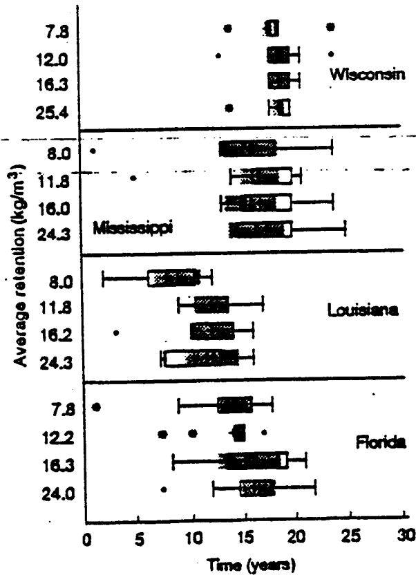
Figure 2. Service-life distributions of states treated with zinc chloride.
