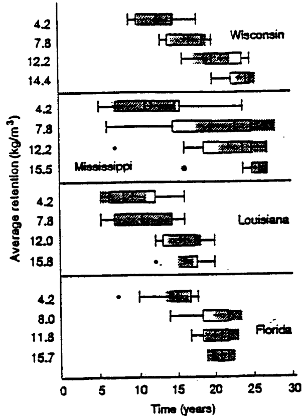
Figure 1. Service-life distributions of states treated with sodium pentachlorophenate.
