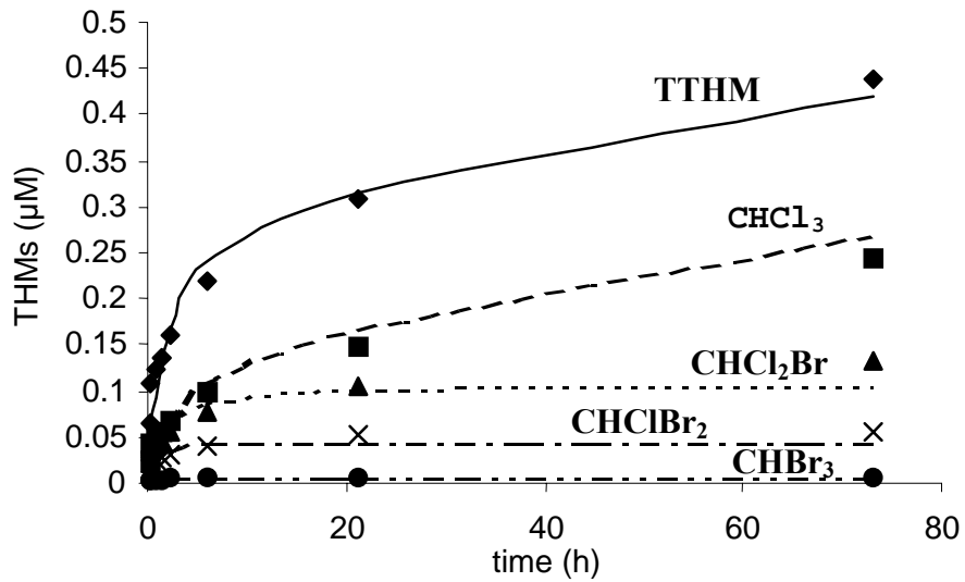
Figure 1. Kinetic production of THM species observed in laboratory batch tests (symbols) and simulated by the mechanistic model (lines) upon chlorination (38 μM) of raw Colorado River water (T = 15° C, pH=7.5, Br = 1.18 μM).
