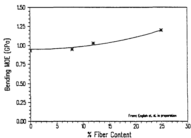
FIGURE 1.—Effect of wastepaper fiber content on woodfiber-plastic composite stiffness.
