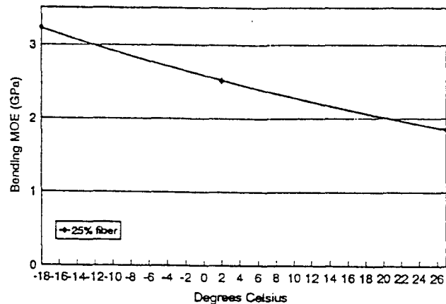
FIGURE 2.—Effect of temperature a HPDE plastic lumber bending stiffness.
