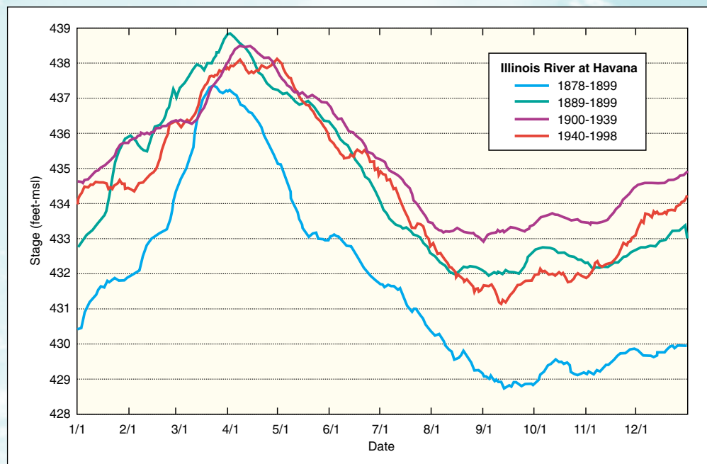
Historical average annual water levels in the Illinois River at Havana.
