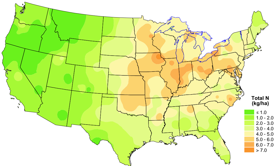
Estimated inorganic nitrogen deposition from nitrate and ammonium, 1999.
