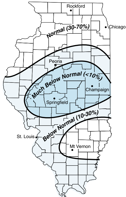
Illinois streamflow levels for May 1-16, 2000.
