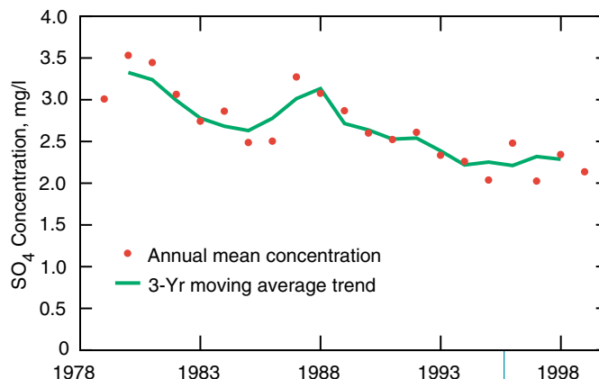
Annual SO 4 concentrations, 1979–1999, NADP/NTN Site IL 11, Bondville, IL.
