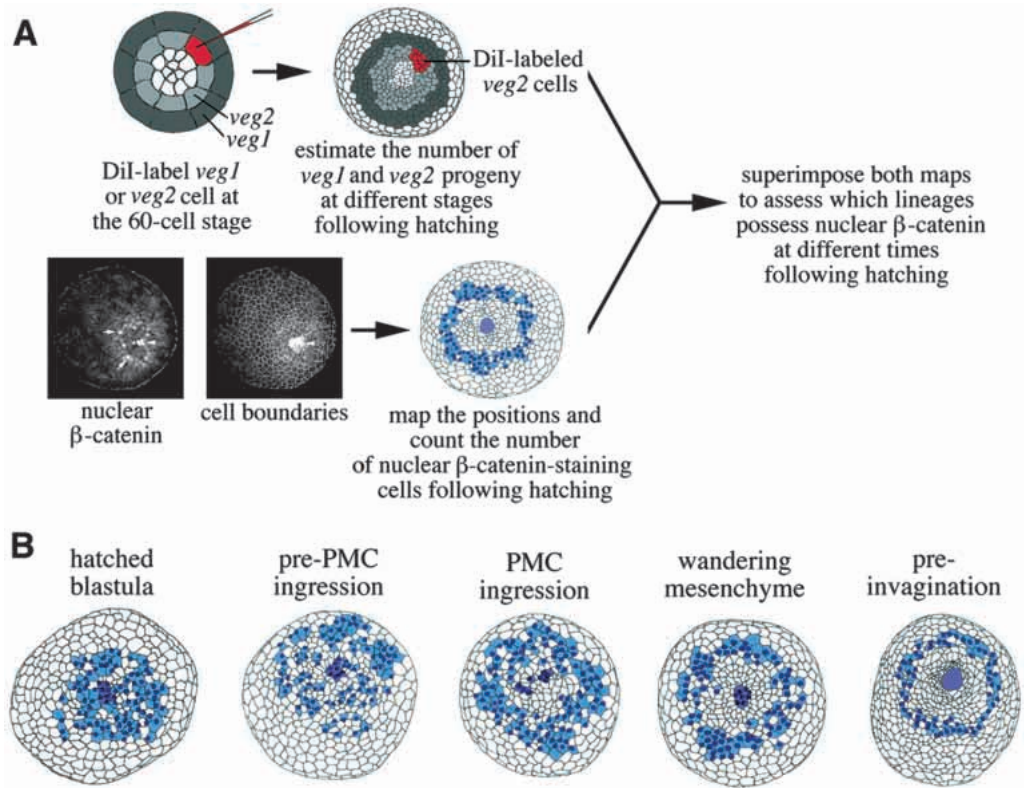
Fig. 2. Pattern of nuclear β-catenin in post-hatching embryos. (A) Schematic showing how we generated stage-specific maps of nuclear β-catenin and determined their relationship to cell lineages. The number of veg1 or veg2 progeny at a given stage was determined by DiI labeling a single veg1 or veg2 cell at the 60-cell stage and by counting the number of labeled descendants at each of several stages after hatching. Since there are eight veg1 or veg2 cells at the 60-cell stage, the total number of veg1 or veg2 cells was estimated by multiplying the number of DiI-labeled cells by 8. These lineage maps were compared to maps of nuclear β-catenin to determine whether the pattern of nuclear β-catenin showed any relationship to micromere, veg2 and veg1 lineages. The small micromeres (arrowheads) were used as a marker of the vegetal pole. (B) Nuclear β-catenin distribution in post-hatching embryos (shown as dark-blue nuclei). Drawings of embryos show a representative pattern of nuclear β-catenin at each of five stages between hatching and invagination of the archenteron. The drawings are vegetal pole views. The position of the small micromeres is indicated by dark-blue cells and the location of β-catenin-positive cells are marked by light-blue cells. Following hatching, progeny of the large micromeres and veg2 cells stochastically downregulate levels of nuclear β-catenin such that all of the PMCs and veg2 cells lack nuclear β-catenin following ingress. This process occurs as β-catenin accumulates in a subset of veg1 cells that form a ring 3-5 cells wide at the wandering mesenchyme stage. Prior to invagination of the archenteron, the circle of veg1 cells that possess nuclear β-catenin narrows to a ring approximately 2 cells wide.
