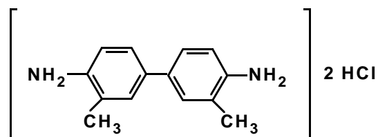
3,3'-DIMETHYLBENZIDINE DIHYDROCHLORIDE
