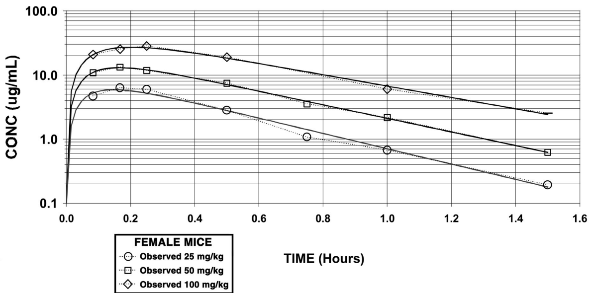
FIGURE M2 Plasma Concentrations of 2-Methylimidazole in Male and Female B6C3F 1 Mice after a Single Gavage Dose of 25, 50, or 100 mg/kg 2-Methylimidazole Solid lines represent the predicted best-fit curves (WinNONLIN ® ) plotted through the observed data points.
