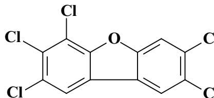
2,3,4,7,8-Pentachlorodibenzofuran PeCDF
