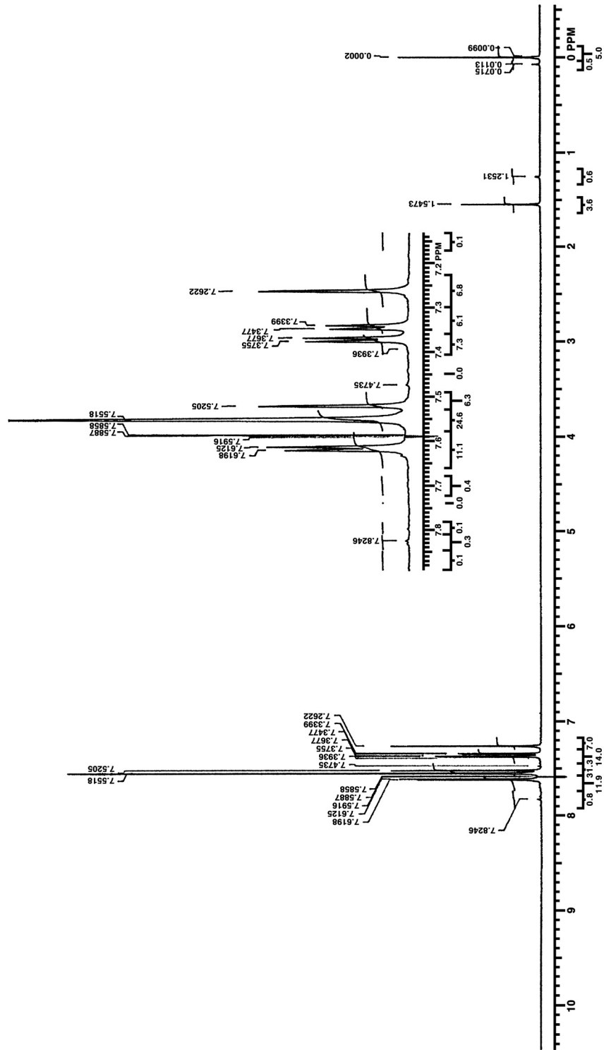
FIGURE C6 Proton Nuclear Magnetic Resonance Spectrum of PCB 126
