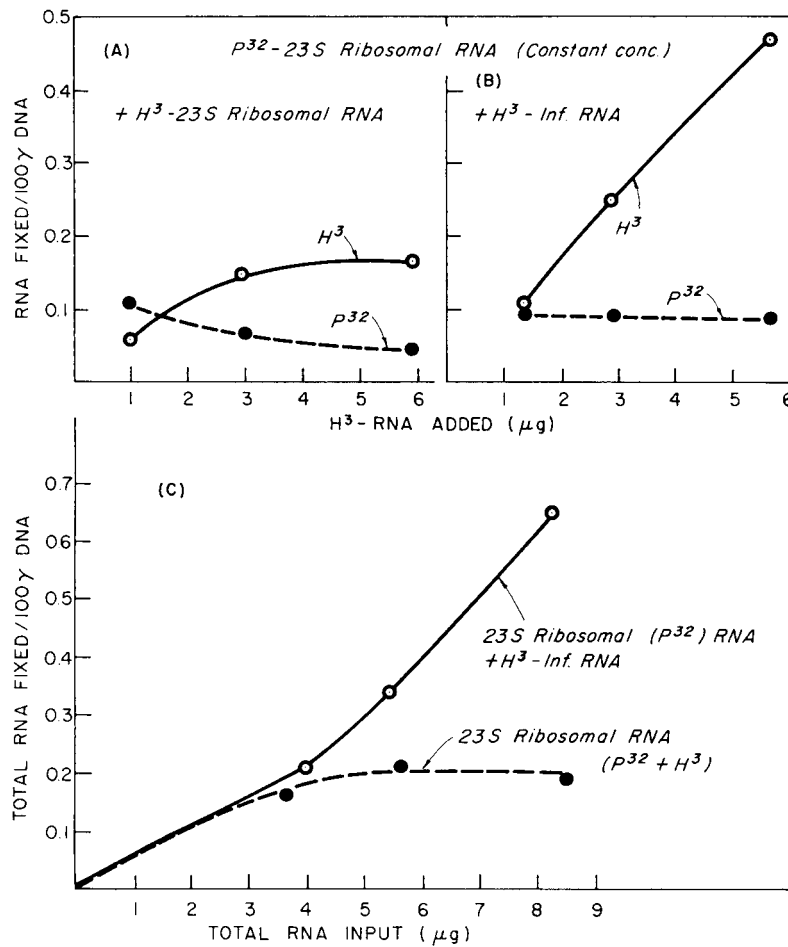
FIG. 5.—Tests for competitive interactions in mixtures of ribosomal and informational RNA molecules. (A) All mixtures contained 63 \mu\text{g}/\text{ml} of heat-denatured E. coli DNA and 2.66 \mu\text{g}/\text{ml} of E. coli P^{32} -23S ribosomal RNA. H^3 -23S ribosomal RNA of E. coli varied as shown. (B) DNA and P^{32} -RNA same as (A) except that H^3 -informational RNA was added in the amounts indicated. (C) The same preparations as (A) and (B). The plot here is total ( P^{32} + H^3 ) RNAase stable counts per 100 \mu\text{g} of DNA as a function of total input of RNA. All incubations during slow cool and equilibrium centrifugations were carried out as described in Figure 1.
