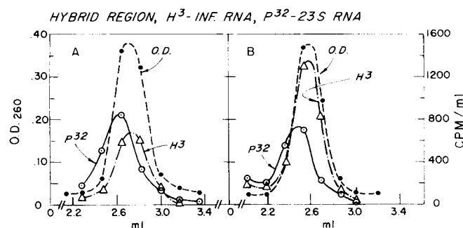
Fig. 4.—Hybrid regions in CsCl gradients of mixtures containing ribosomal and informational RNA. Both incubation mixtures contain 63 \mu\text{g}/\text{ml} of heat-denatured E. coli DNA and 2.66 \mu\text{g}/\text{ml} of E. coli P^{32} -23S RNA. (A) contained in addition 2.9 \mu\text{g} of H^3 -informational RNA and (B) 5.7 \mu\text{g} of H^3 -informational RNA per ml. Details of incubations and centrifugations are as in Figures 1 and 2.
