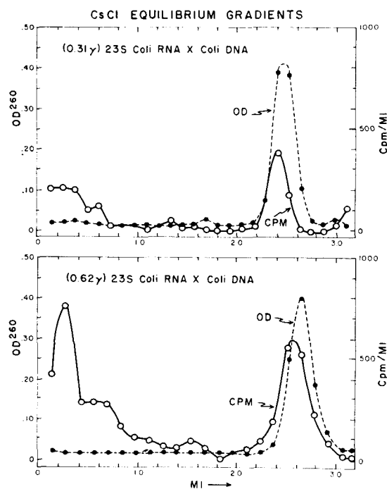
FIG. 1.—CsCl equilibrium density gradient profiles. Buffer used was TMSV (0.03 M tris, pH 7.3; 0.001 M MgCl 2 ; 0.3 M NaCl 0.005 M EDTA. Both contained 71 μg per ml of heat-denatured E. coli DNA. Upper contained 0.31 μg and the lower 0.62 μg of P 32 -23S RNA (6.7 × 10 4 cpm/μg) of E. coli . Reaction mixtures slow (ca. 13 hr) cooled from 55°C to 33°C. Mixtures were then brought to a density of 1.73 with CsCl and a total volume of 3 ml. They were centrifuged for 52 hr at 33,000 rpm and 25°C.
