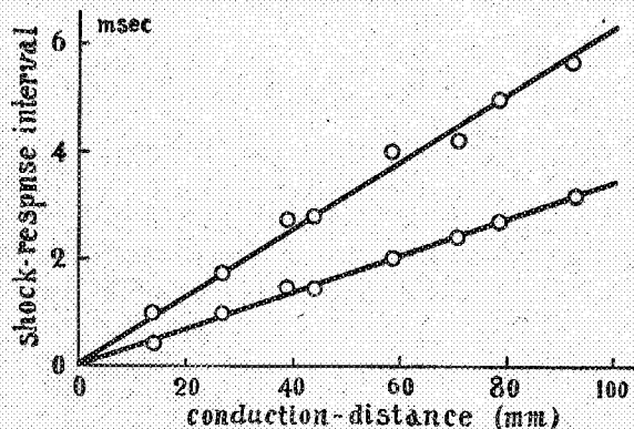
Fig. 7. Shock-response interval as a function of conduction-distance in a 2-fibre preparation. Diameter of the fibres, 12 and 6 \mu (See Series 5 of the photographic records).
