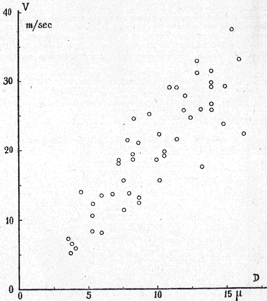
Fig. 4. Conduction-rate V (ordinates) plotted against fibre-diameter D. Data from 49 single fibres of the bull frog. 24^\circ \text{C} .
