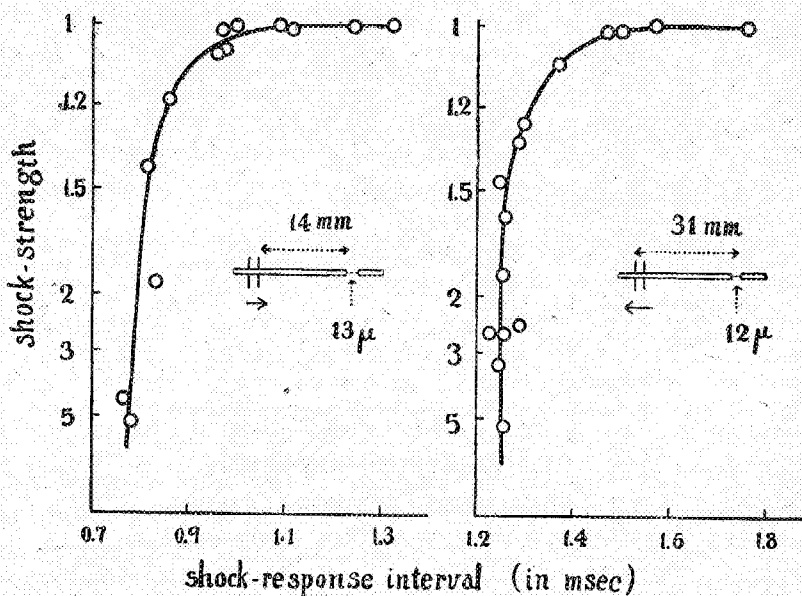
Fig. 2. Experimental results showing the relation between the shock-strength and the shock-response interval in single-fibre preparations. Conduction-distance, direction of the induction current and the fibre-diameter are shown in the diagram in each case.
