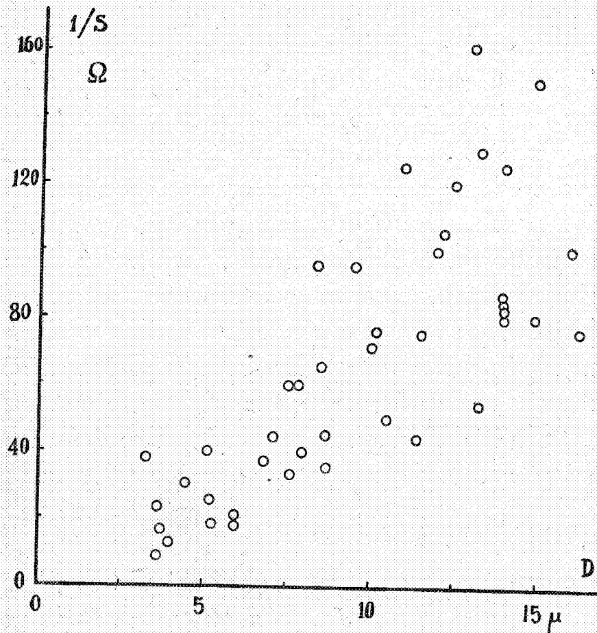
Fig. 5. Reciprocal of the threshold strength 1/S (ordinates) plotted against fibre-diameter D . Bull frog's single fibres.
