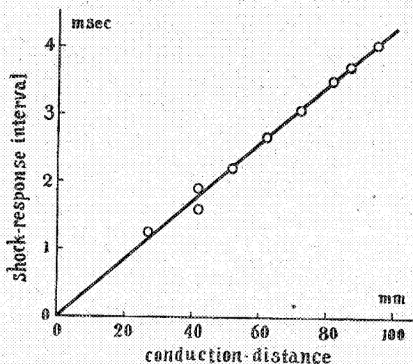
Fig. 3. Demonstration of linearity of the nervous conduction in a single nerve fibre. Diameter of the fibre, 8 \mu .
