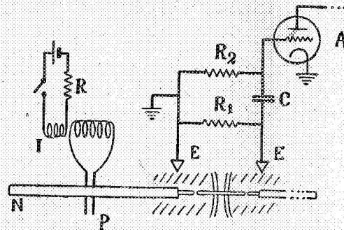
Fig. 1. Diagram showing the experimental arrangement. N, nerve; P, platinum electrodes; I, inductorium; R, resistance; R 1 , 50 (or 500), R 2 , 300 (or 500) kilo-ohms; C, condenser of 2 microfarads; E, non-polarizable electrode; A, amplifier.
