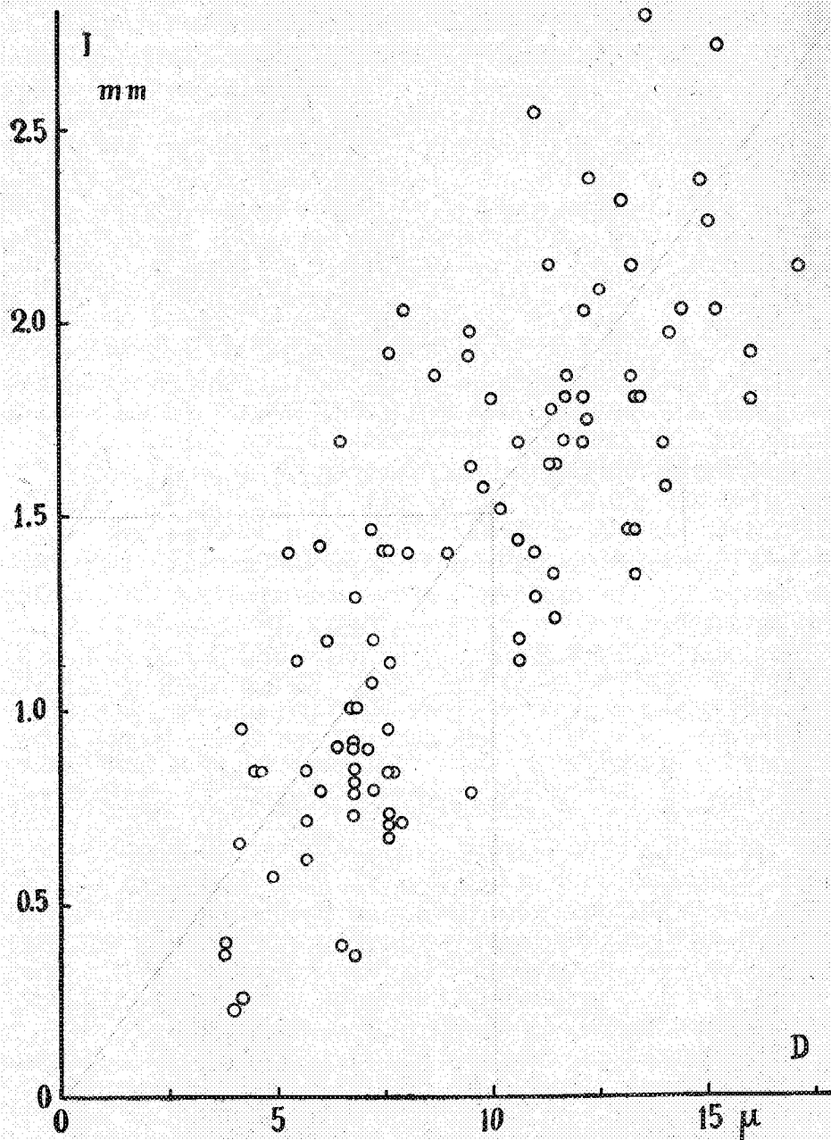
Fig. 6. Distance between two neighboring nodes of Ranvier I plotted against fibre-diameter D. Data from 100 fibres of the bull frog.
