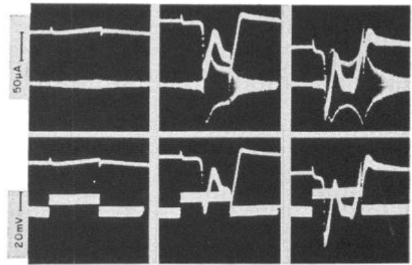
FIG. 7. An example of the records obtained by the method of filtered a.c. for measuring the conductance of the squid axon membrane under voltage-clamp. Temperature was 7.5°C. The length of the internal current-electrode was 15 mm and that of the internal potential-electrode 5 mm. The membrane current is expressed in the total value, and not in values per unit area, because the partitions and the lateral ground electrodes in fig. 1 were not present in this experiment. Axon diameter, 500 \mu .
