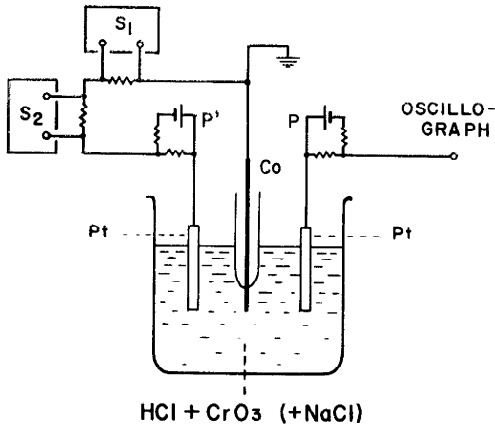
FIG. 1. Experimental setup used to demonstrate 'abolition of the action potential' and 'subthreshold responses' in the cobalt-electrode system. Co , cobalt wire of about 1 mm in diameter enclosed partly in a glass tubing. Pt , platinum wire for recording potential variations ( right ) and for applying current pulses to the cobalt wire ( left ). S 1 and S 2 , stimulus isolation unit (Grass). P and P' , 3 volt batteries and potential dividers for compensating the potential difference between the platinum and cobalt wire.
