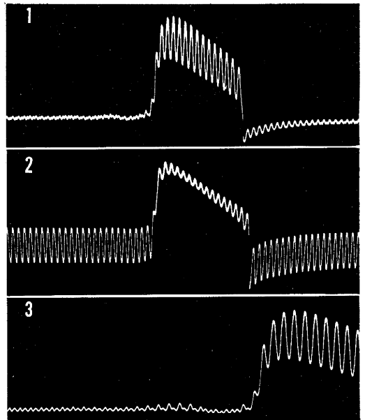
FIG. 4. Demonstration of 'impedance loss during activity' in the cobalt-electrode system. An a.c. Wheatstone bridge was used to reduce the amplitude of the a.c. component before the start of a 'response' ( top and bottom ) or during 'activity' ( middle ). Bottom record was taken at higher film speed.
