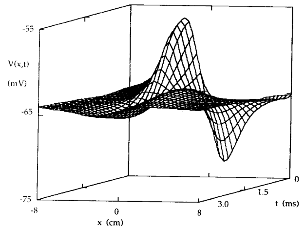
Fig. 7. A three-dimensional plot of the subthreshold response of the nerve fiber to electromagnetic stimulation ( V_o = 30 V). The vertical axis is the transmembrane potential in the fiber, and the horizontal axes represent the distance along the fiber x and the time after the capacitor was discharged t .
