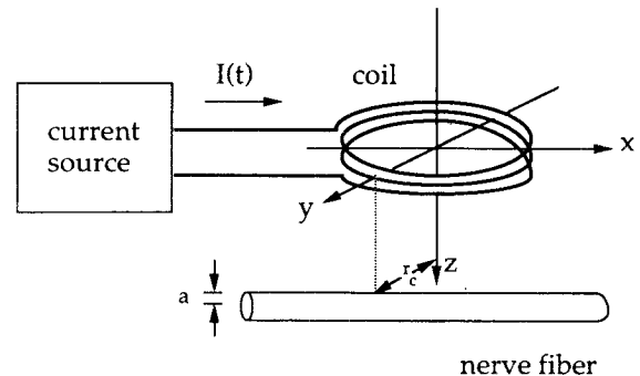
Fig. 1. A schematic diagram showing the experimental apparatus for stimulating a nerve using electromagnetic induction. A current I(t) is passed through a coil placed near a nerve fiber; the induced electric field stimulates the nerve. The nerve lies parallel to the x axis at y = r_c and z = 1.0 cm. The coil radius is also r_c ; the fiber radius is a .
