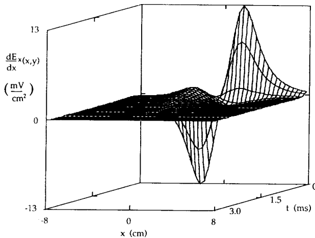
Fig. 6. The source term \partial \epsilon_x / \partial x as a function of x and t , evaluated along the length of the nerve fiber. This function represents the gradient of the electric field along the line y = r_c , shown in Fig. 3(b), modulated in time by the current waveform shown in Fig. 5(b).
