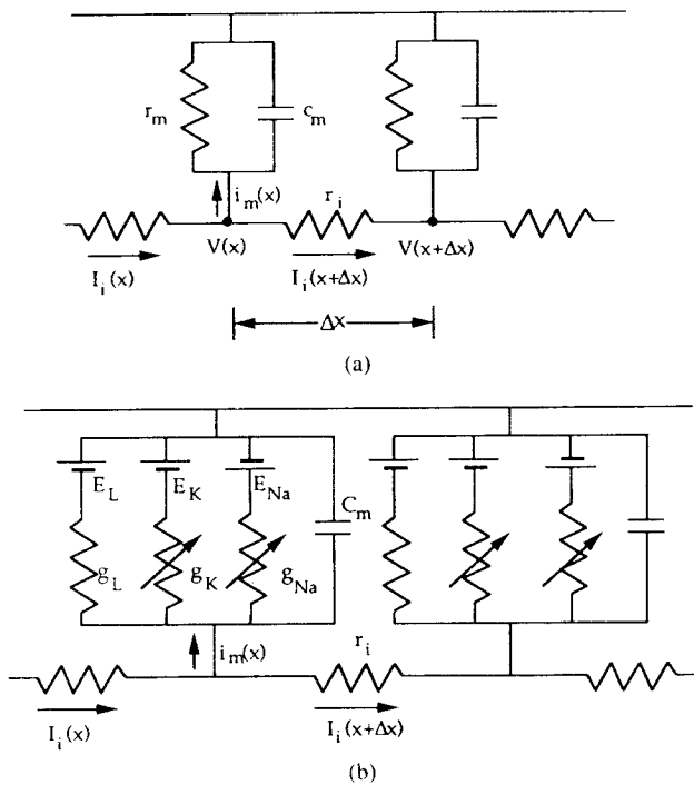
Fig. 2. (a) An electrical circuit representing the passive cable. The intracellular space is modelled by a resistance per unit length r_i , the membrane by a resistance times unit length r_m and capacitance per unit length by c_m . The extracellular potential is assumed to be zero. The axial intracellular current I_i(x) is related to the intracellular potential V(x) by Ohm's law, and related to the membrane current per unit length, i_m(x) by the equation of continuity. (b) An active cable with Hodgkin-Huxley membrane. The membrane is now represented by three voltage and time dependent conductances, representing the sodium, potassium, and leakage channels [22].
