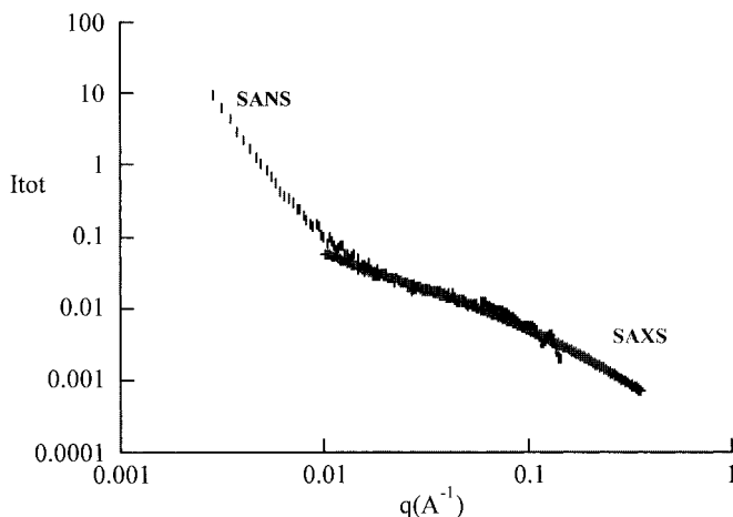
Fig. 3. SAXS (+) and SANS (I) scattering as a function of momentum transfer q . The SAXS response has been shifted vertically to coincide with the SANS intensity scale.
