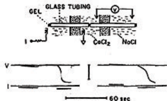
Fig. 9. Demonstration of cooperativity of the \text{Na}^+ - \text{Ca}^{2+} exchange in cross-linked Na-polyacrylate gel. First, the gel, in glass tubing (1 mm in inside diameter and 30 mm in length), was equilibrated with 40 mM NaCl solution. Next, by gently breaking the glass tubing, a very short segment of the gel surface in the middle was exposed to 100 mM \text{CaCl}_2 solution. Subsequently, a constant current pulse was delivered between the middle and left-hand pools of solutions, and the continuous potential change developed across the exposed gel surface in the middle was recorded (see the trace marked V). The current intensities (indicated by the trace marked I) were, from the left, -0.3, -0.6, +0.6, and -0.6 mA. Note that the rapid change in the potential is preceded by a period of gradual change. Bar: 1 V.
