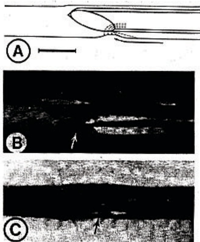
Fig. 7. Demonstration of direct connection of the filamentous material in the ectoplasm with the axolemma of a fresh giant axon. A: Schematic diagram illustrating suction of the protoplasm into a glass pipette inserted into a squid giant axon. B, C: Photographs taken from a fresh excitable axon, placed between a polarizer and an analyzer in a crossed position, showing strong birefringence of the protoplasmic gel in the vicinity of the rear end of the orifice of the glass pipette. The broken lines in diagram A show the orientation of the filaments revealed by the birefringence of the protoplasm (from Metuzals and Tasaki [42]).
