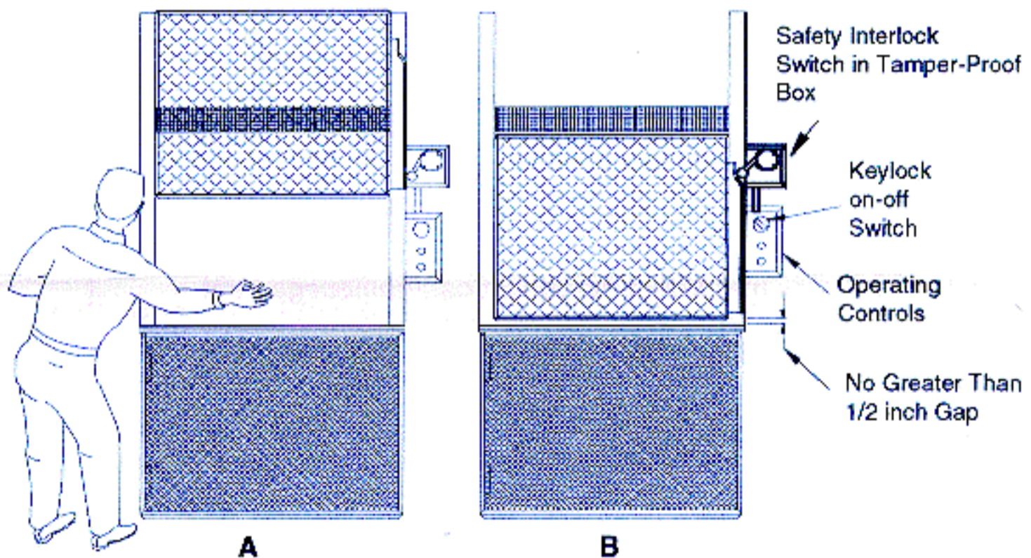
Figure 2. Sample Interlocked Sliding Gate: Two gate positions are shown: (A) open for loading (potentially hazardous) and (B) closed for operating (safe). The safety interlock switch opens and closes electrical contacts that control power to the baler ram depending on the position of the gate. Tampering, misadjustment, or wear of the safety interlock switch can allow the gate opening to exceed 1/2 inch (maximum). Note that the baler shown also has a key-locked power control that prevents baler operation when the key is removed and kept by an authorized person.
