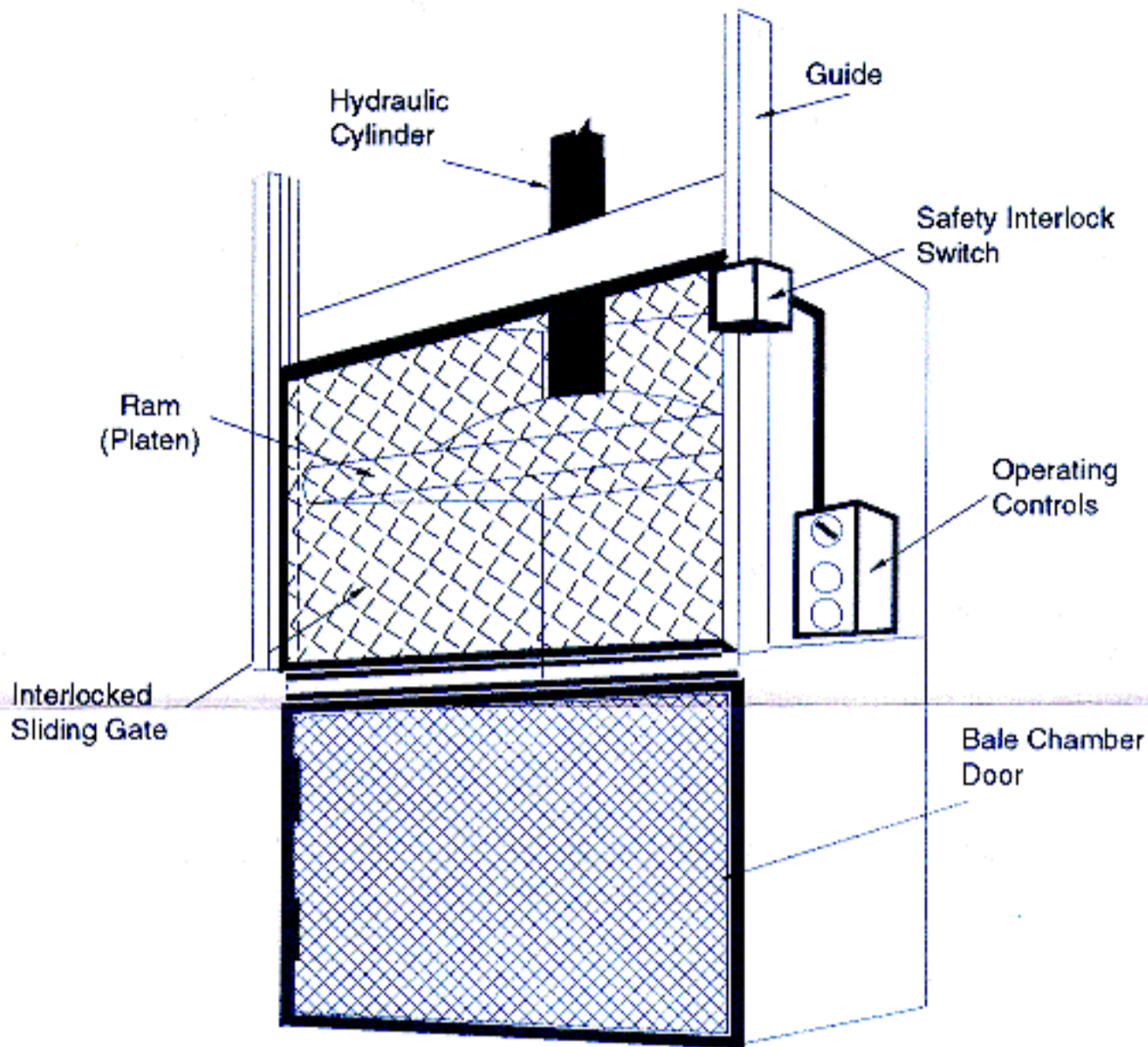
Figure 1. Vertical Downstroke Baler: Basic components
