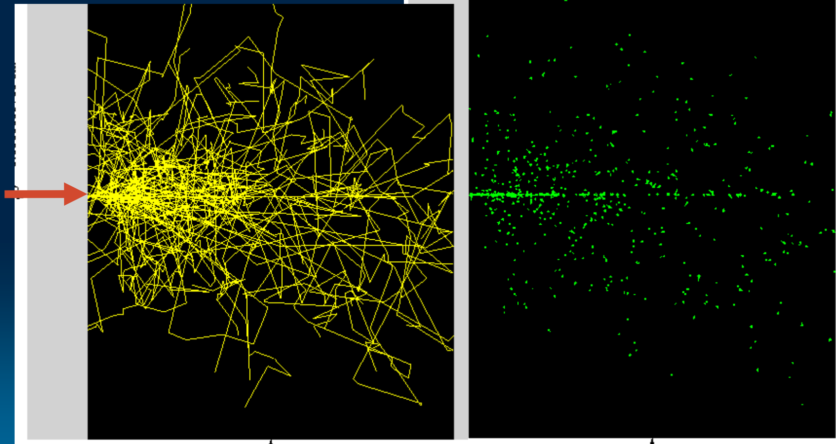
Scattered photons
