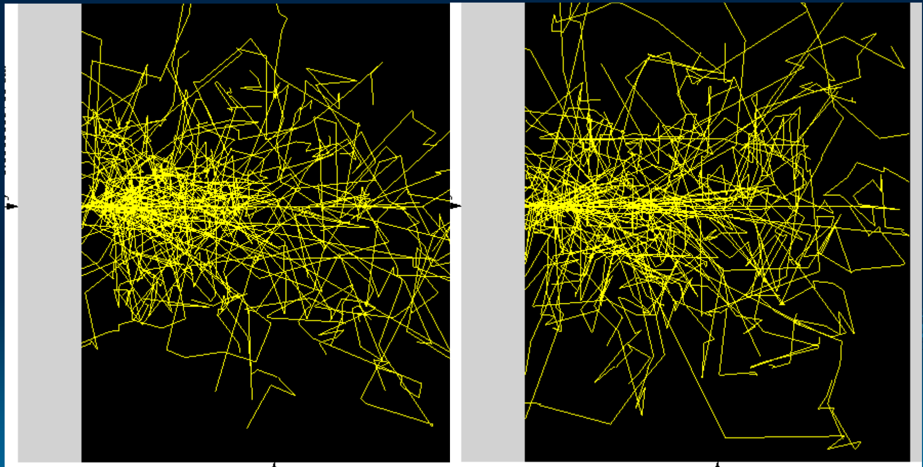
1 st 100 photons
