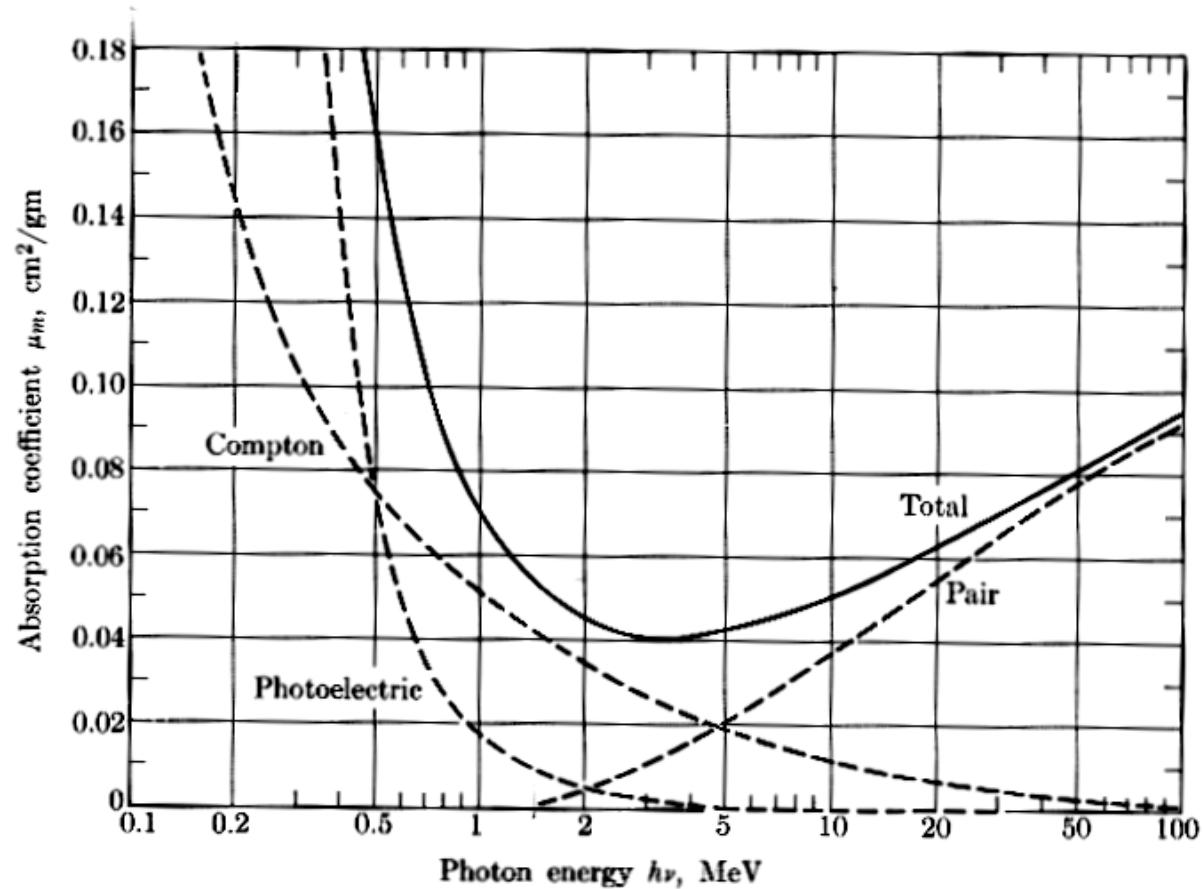
Total mass-absorption coefficients for gamma rays in lead and the contributions from the photoelectric effect, the Compton effect, and pair production.
