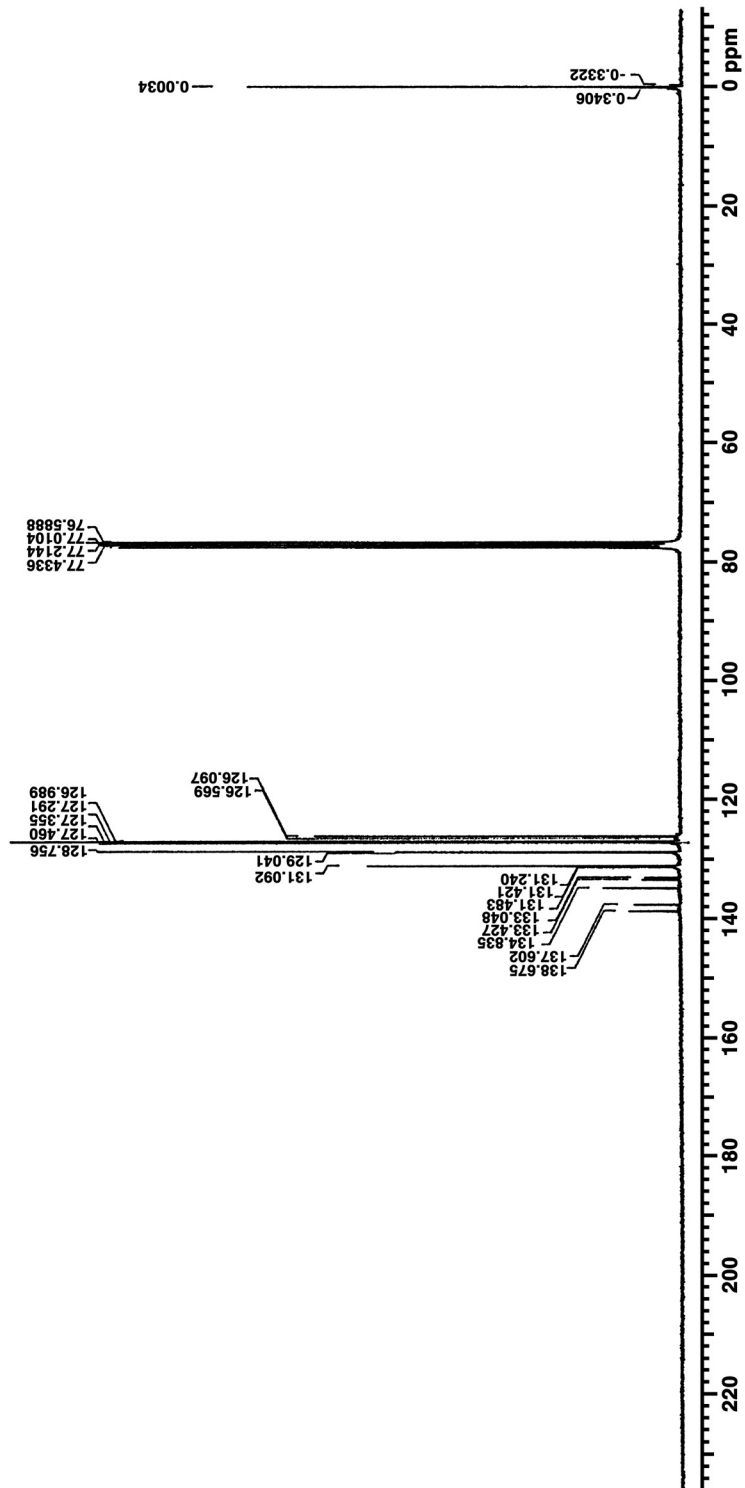
FIGURE C2 Carbon-13 Nuclear Magnetic Resonance Spectrum of PCB 126
