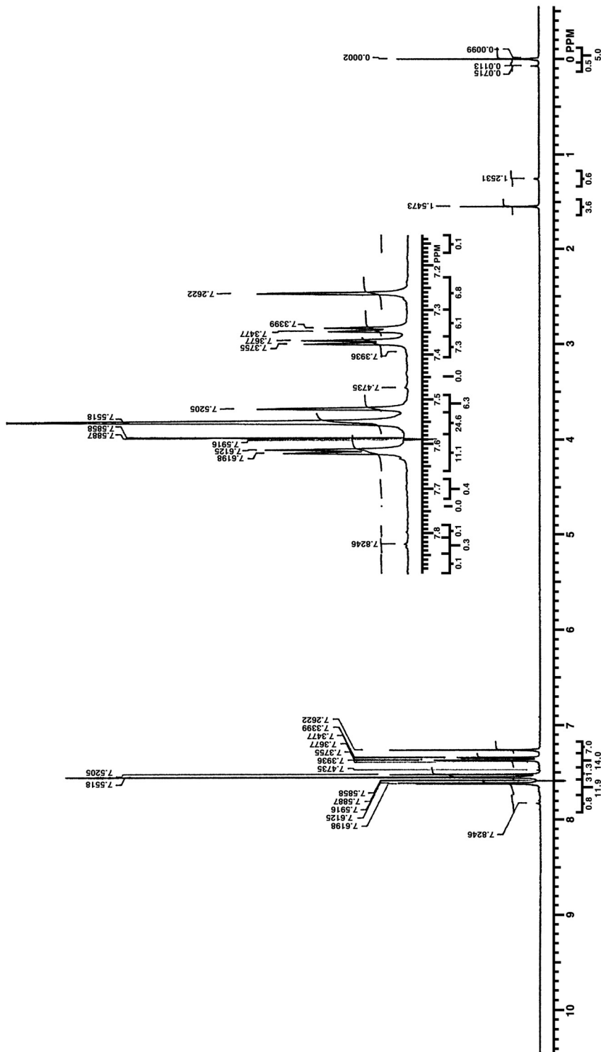
FIGURE C1 Proton Nuclear Magnetic Resonance Spectrum of PCB 126
