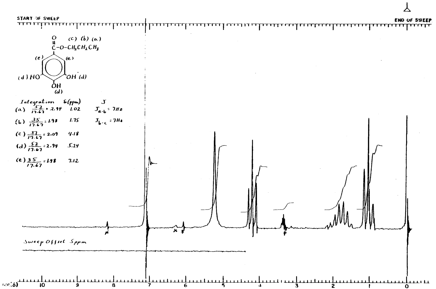
Figure 8. Nuclear Magnetic Resonance Spectrum of Propyl Gallate (Lot No. 831)
