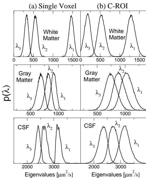
Fig. 16. Bootstrap estimate of the probability density function of diffusion tensor eigenvalues within (a) a single voxel and (b) corresponding ROIs (the white matter ROI was ICI, shown in Fig. 13). It is evident that the ROI estimates of variability and those of a single voxel disagree. This disparity points to a significant intrinsic variability of the rotationally invariant quantities.
