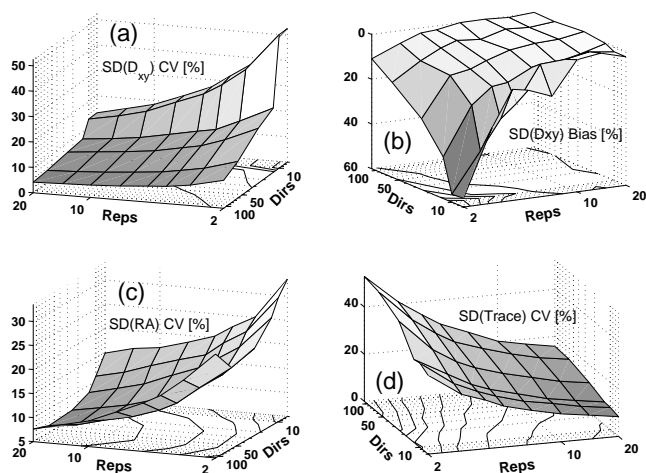
Fig. 6. How the quality of the bootstrap estimates depends on the number of different gradient directions and the number of repetitions for each of the directions. Figures (a), (c), and (d) show the dependence of the precision of a given bootstrap estimate on a given statistic, \theta_B , expressed through CV = SD(\theta_B)/\theta_B . The statistics used are (a) standard deviation of an off-diagonal element, SD(D_{xy}) ; (c) standard deviation of relative anisotropy, SD(RA) ; and (d) standard deviation of the trace, SD(\text{trace}) . Figure (b) shows the bias of the estimates, bias = (\theta_B - \theta_B^{\text{true}})/\theta_B^{\text{true}} expressed as a percent.
