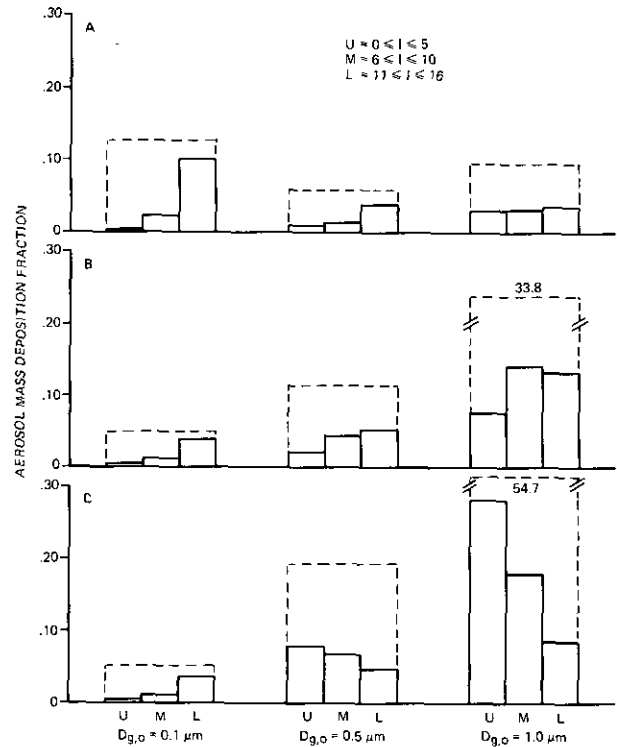
FIGURE 14. Influence of RH profile and D_{g,0} on (---) total dose and (—) regional distribution of \text{NH}_4\text{HSO}_4 aerosols inhaled at Q = 60 \text{ L/min} : U = upper, M = middle, and L = lower airways. I denotes airway generation. (A) nonhygroscopic particle behavior included for comparison; (B) 90–99.5% RH; (C) 99.5% RH.
