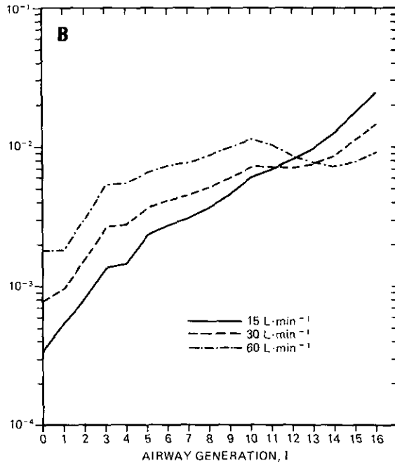
FIGURE 7. Influence of inspiratory flow rate on the relative percent dispersion of the total dose of ambient 0.5- \mu\text{m} D_{g,0} H 2 SO 4 particles for different RH profiles in the TB tree: (A) nonhygroscopic particle behavior included for comparison; (B) 90–99.5% RH; (C) 99.5% RH.
