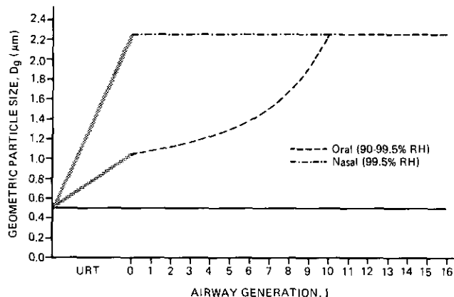
FIGURE 8. Change in diameter of a submicrometer ( D_{g,0} = 0.5 \mu\text{m} ) \text{H}_2\text{SO}_4 particle for various breathing modes: (—) nonhygroscopic particle behavior included for comparison. URT denotes upper respiratory tract.
