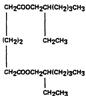
Di(2-ethylhexyl)adipate
