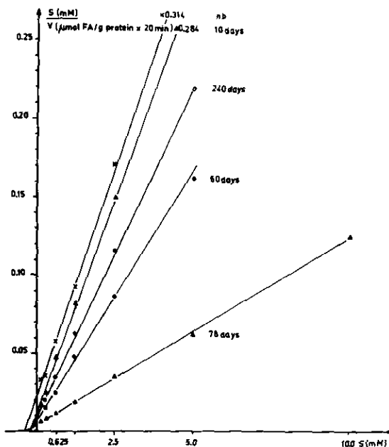
FIGURE 15. Endernyi-Kwong plot of same values given in Fig. 14.
