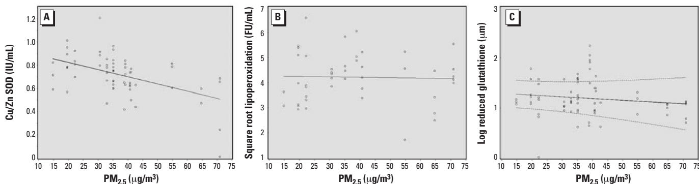
Figure 3. Cu/Zn SOD (A), LPO (B), and GSH (C) according to PM 2.5 exposure ( \mu\text{g}/\text{m}^3 ; based on our GAMMs) among patients in the soy oil group. Solid line, estimated smooth function; dashed lines, pointwise 95% CIs; circles, partial residuals. We suppressed CIs in cases where we estimated one smooth function to be linear or any variance component to be (almost) zero, because the covariance matrix is then singular and cannot be inverted for construction of the variability bands.
