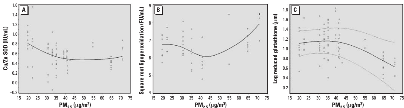
Figure 2. Cu/Zn SOD (A), LPO (B), and GSH (C) according to PM 2.5 exposure ( \mu\text{g}/\text{m}^3 ; based on our GAMMs) among patients in the fish oil group. Solid line, estimated smooth function; dashed lines, pointwise 95% CIs; circles, partial residuals. We suppressed CIs in cases where we estimated one smooth function to be linear or any variance component to be (almost) zero, because the covariance matrix is then singular and cannot be inverted for construction of the variability bands.
