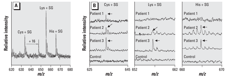
Figure 7. MALDI-TOF spectra of amino acid-SG adducts in pronase digests of rHSA (A) and amino acid-SG adducts in pronase digests of HSA (B) from S. chartarum -exposed and control patients.
