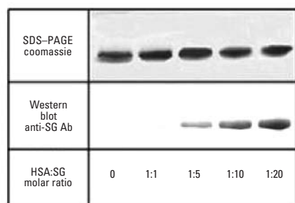
Figure 4. SDS-PAGE and Western blots of HSA incubated with different concentrations of SG (3 \mu g protein/lane). Western blots were developed with affinity-purified anti-SG antibody (Chung et al. 2003).
