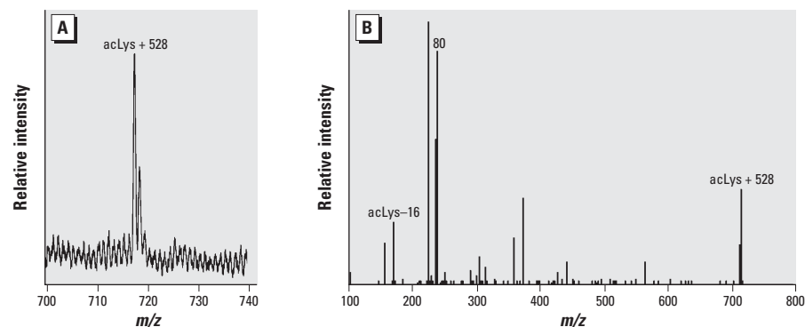
Figure 5. (A) Portion of the MALDI-TOF mass spectrum of N - \alpha -acetyl-L-lysine (acLys) incubated with equimolar concentration of SG. A peak is detected at m/z 716.8. (B) ESI MS-MS spectrum of the ions at m/z 716.8.
