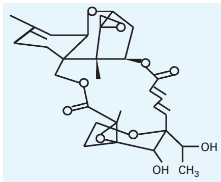
Figure 1. Structure of SG. Abbreviations: OH, hydroxyl group; \text{CH}_3 , methyl group.
