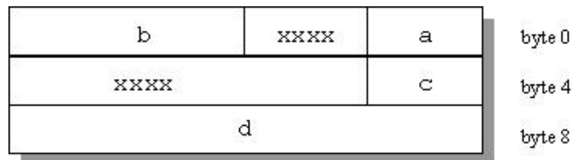
Figure 14.1. Internal Padding in a Structure
