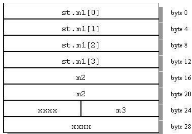
Figure 14.2. Tail Padding in a Structure
