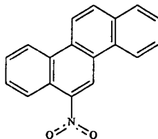
6-Nitrochrysene [7496-02-8]
