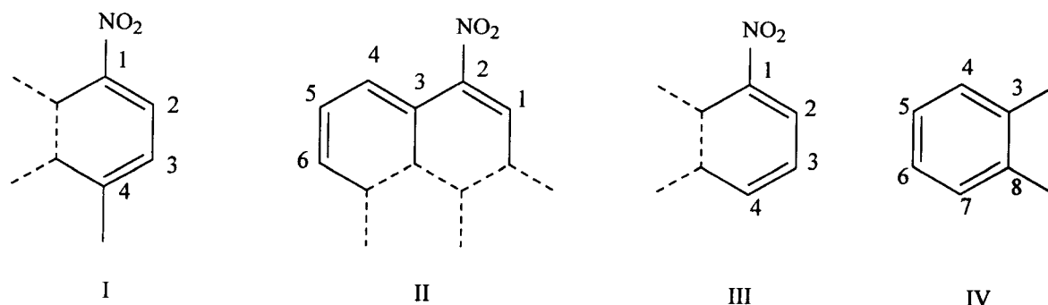
Figure 6-2. Fragments Responsible for the Mutagenicity of Nitroarenes
