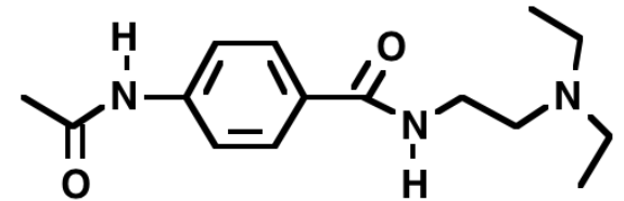
N-acetylprocainamide
