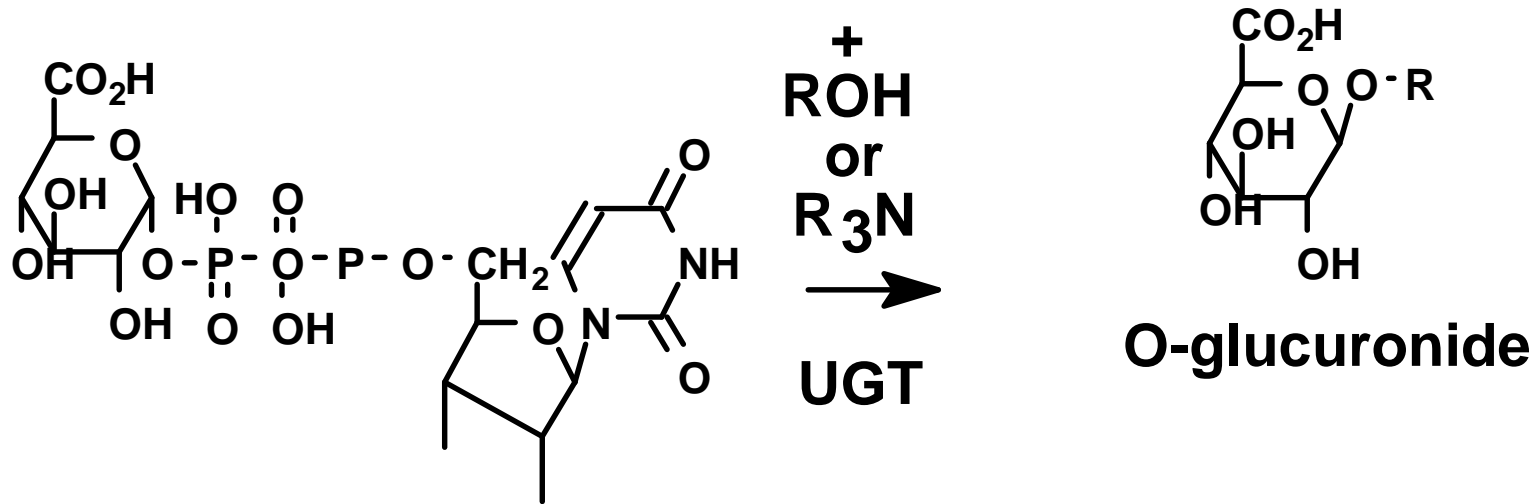
UDP- \alpha -D-glucuronic acid
