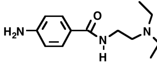
procainamide
