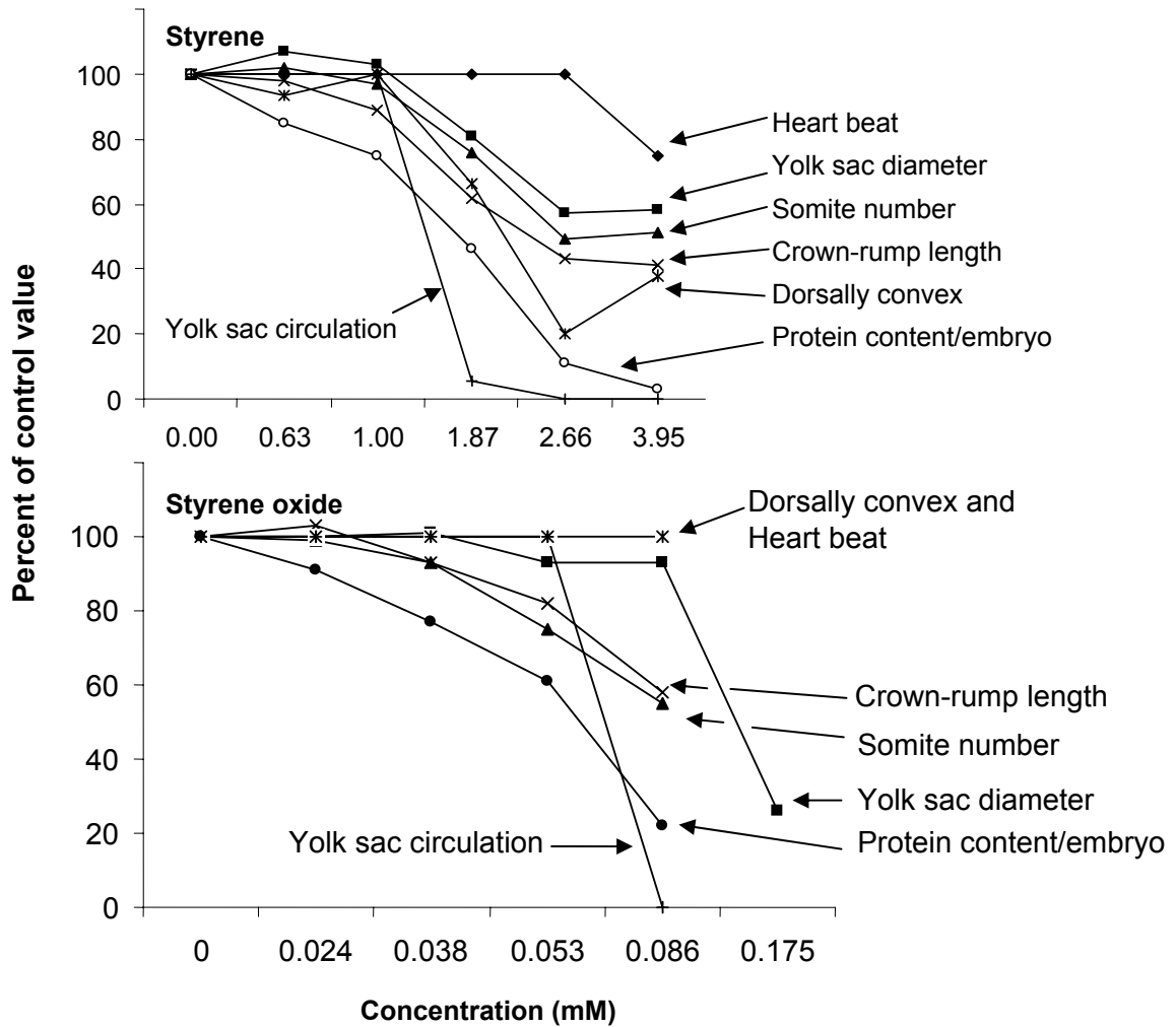
Figure 3. Concentration–response relationship of styrene and styrene oxide in rat whole embryo culture. Figure drawn from the data of Brown-Woodman et al. (96).
