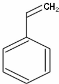
Figure 1. Structure of styrene
