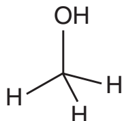
Figure 1. Chemical structure of methanol
