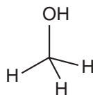
Figure 1-1: Chemical Structure of Methanol
