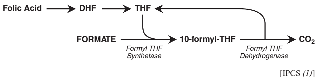
Figure 2-2: Metabolism of Formate through the Folate Pathway
