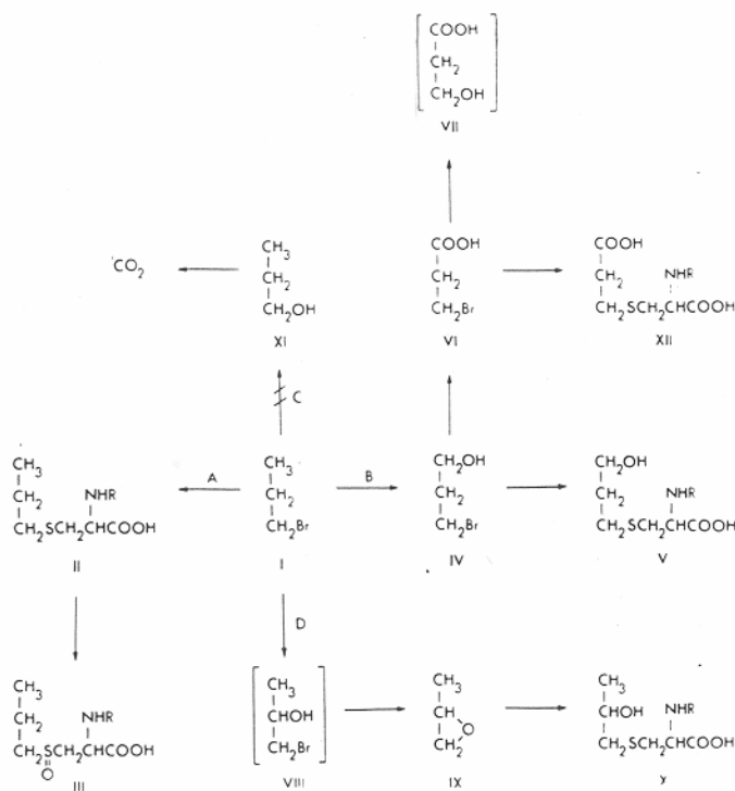
Figure 2-1. Possible metabolic pathway for 1-BP in the rat. Compounds in parantheses were not isolated in urine. Copied from Jones and Walsh (1979).
