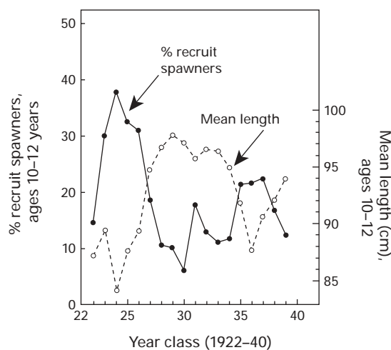
Lower part: Growth and maturation of Icelandic cod, 1932-50 (redrawn from Jónsson, 1954).
