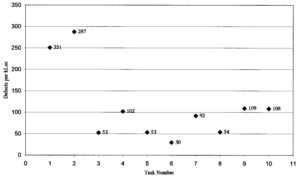
Figure 1. Defect rates for all C++ tasks
