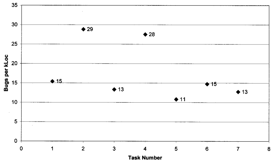
Figure 3. Bugs (test defects) for relevant C++ tasks
