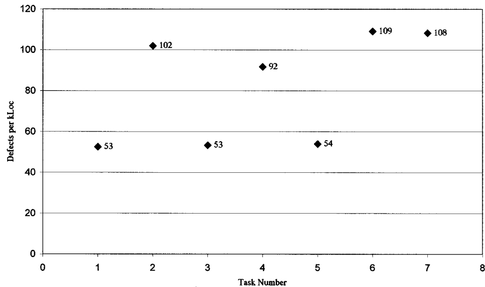
Figure 2. Defects for relevant C++ tasks
