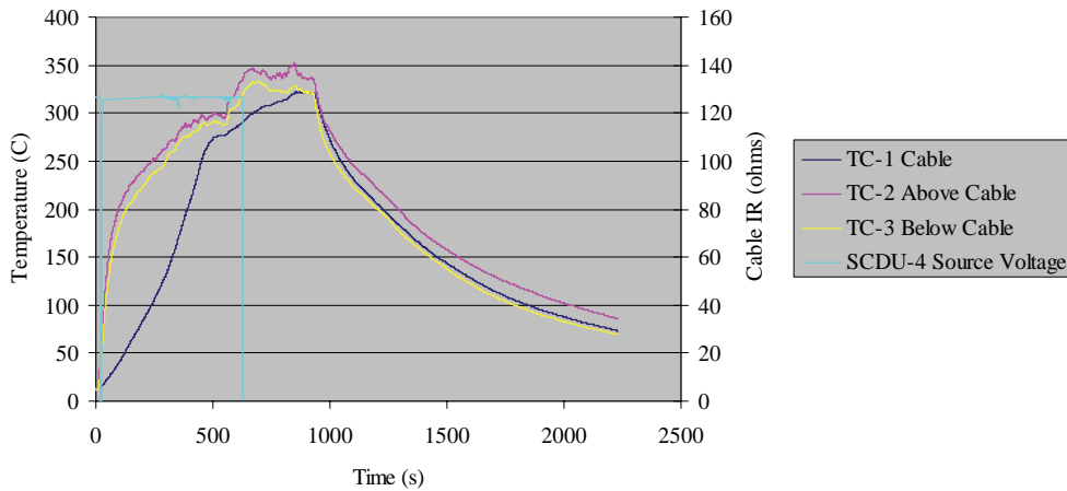
Figure 6.33: Thermal response and electrical performance for the single 3/C PVC/PVC cables at Location G during IT-3.
