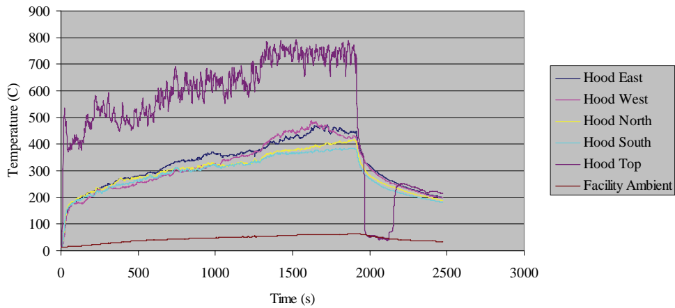
Figure 6.57: Hood temperatures measured during IT-9.
