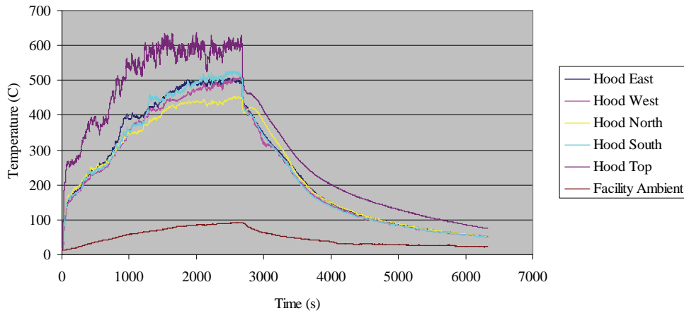
Figure 6.21: Hood temperatures measured during IT-1.
