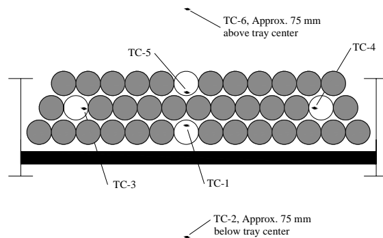
Figure 3.7: TC complement for the random fill tray in IT-1.
