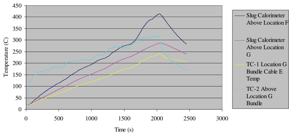
Figure 6.54: Temperature response for the slug calorimeters and the cable bundle at Location G during IT-8.
