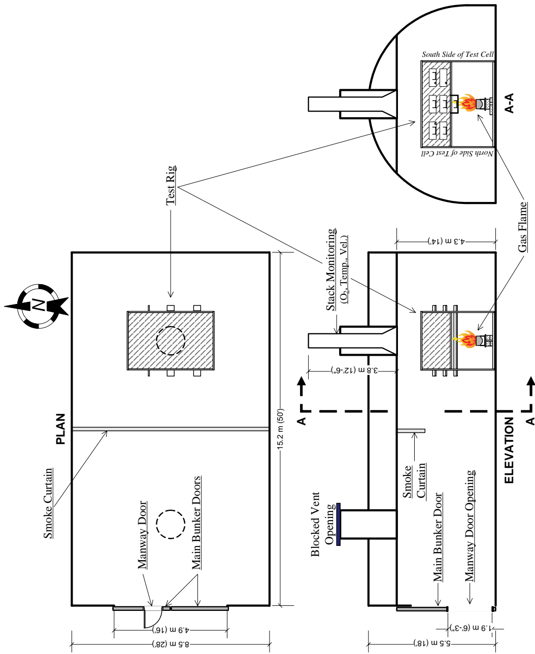
Figure 2.11: Schematic representation of the CAROLIFRE Intermediate-Scale Test Structure (or 'rig') located within the outer test facility.
