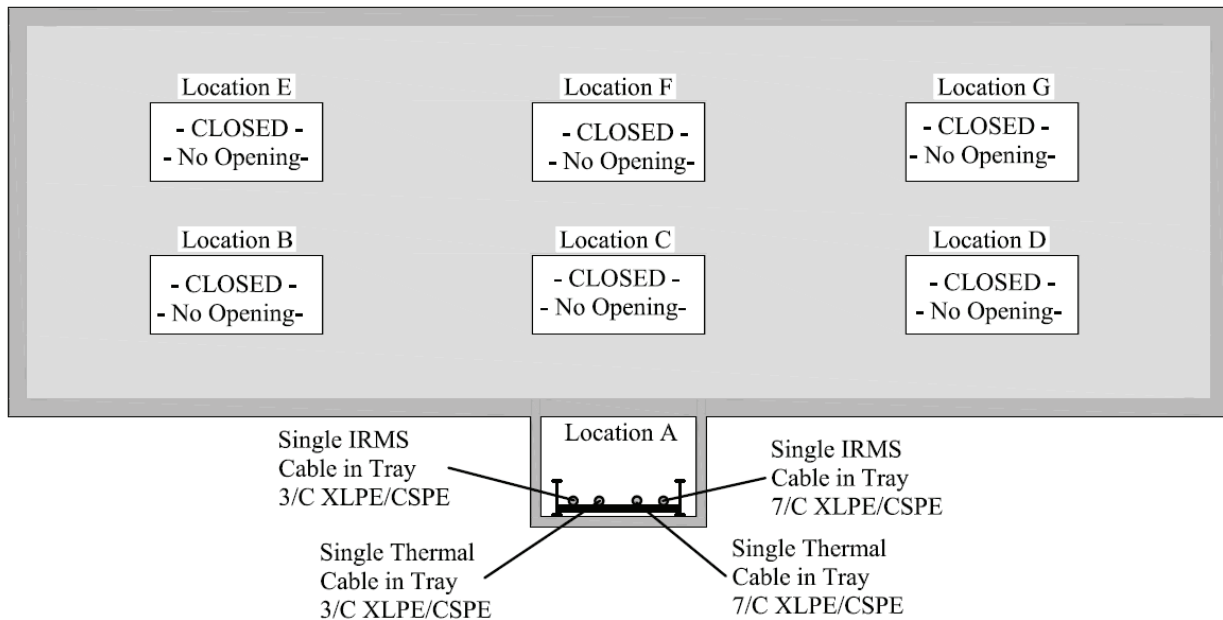
Figure 6.1: Illustration of the test conditions for tests IP-1 and IP-2.
