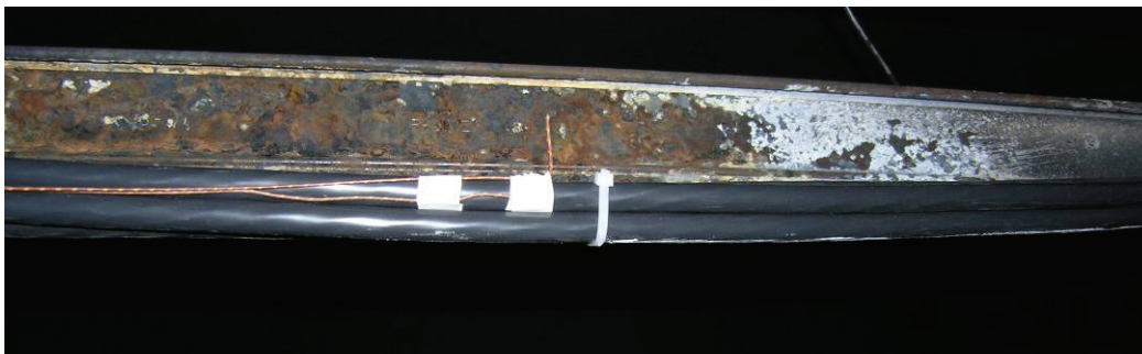
Figure 6.64: Photograph of the horizontal air-drop cable bundle from IT-11.
