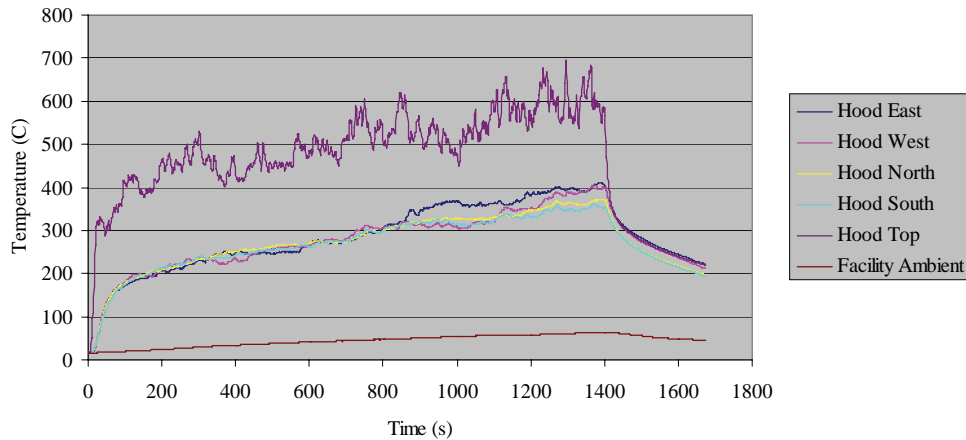
Figure 6.48: Hood temperatures measured during IT-7.
