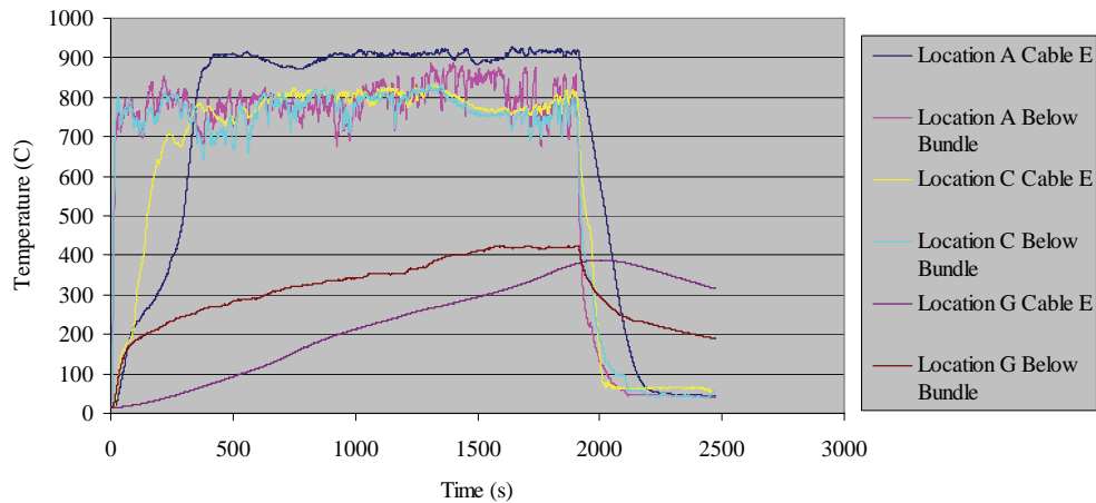
Figure 6.58: Temperature response data for the cable bundles at Locations A, C and G during IT-9.
