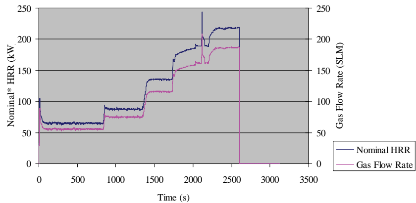
Figure 6.2: Fuel gas measured flow rate and nominal heat release rate for IP-1.
