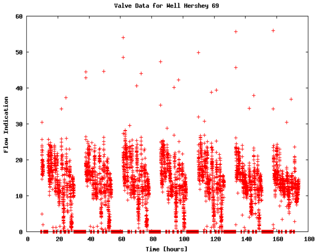
Plot 1: A week-long wireless test
