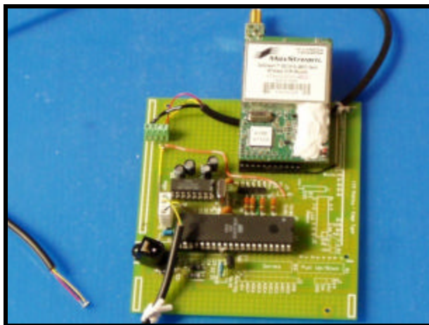
Photograph 1: Microcontroller and radio modem circuits
