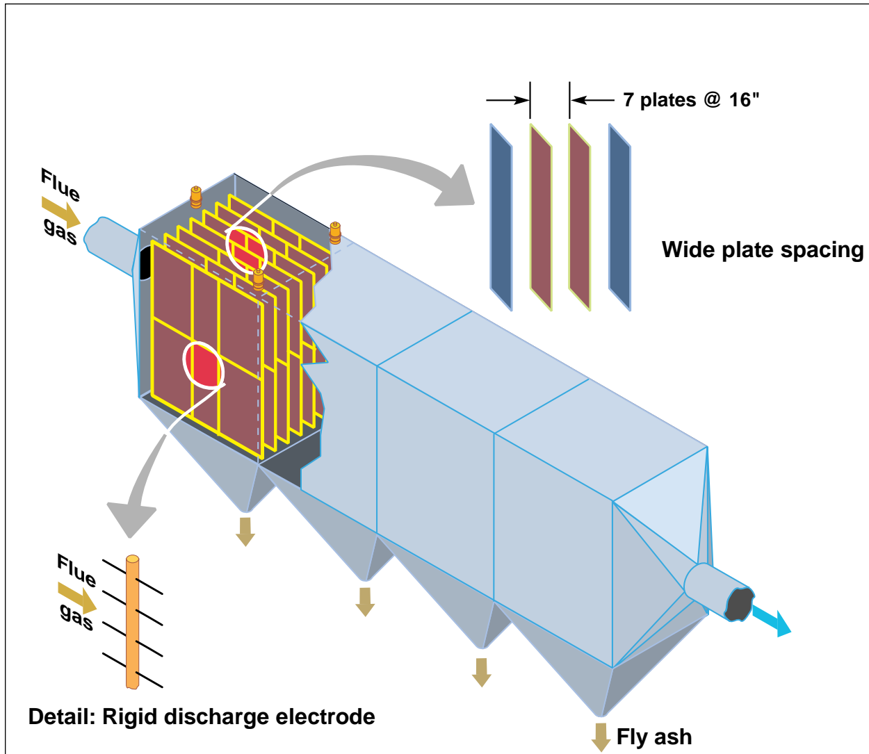
Figure 4 -- Electrostatic Precipitator
