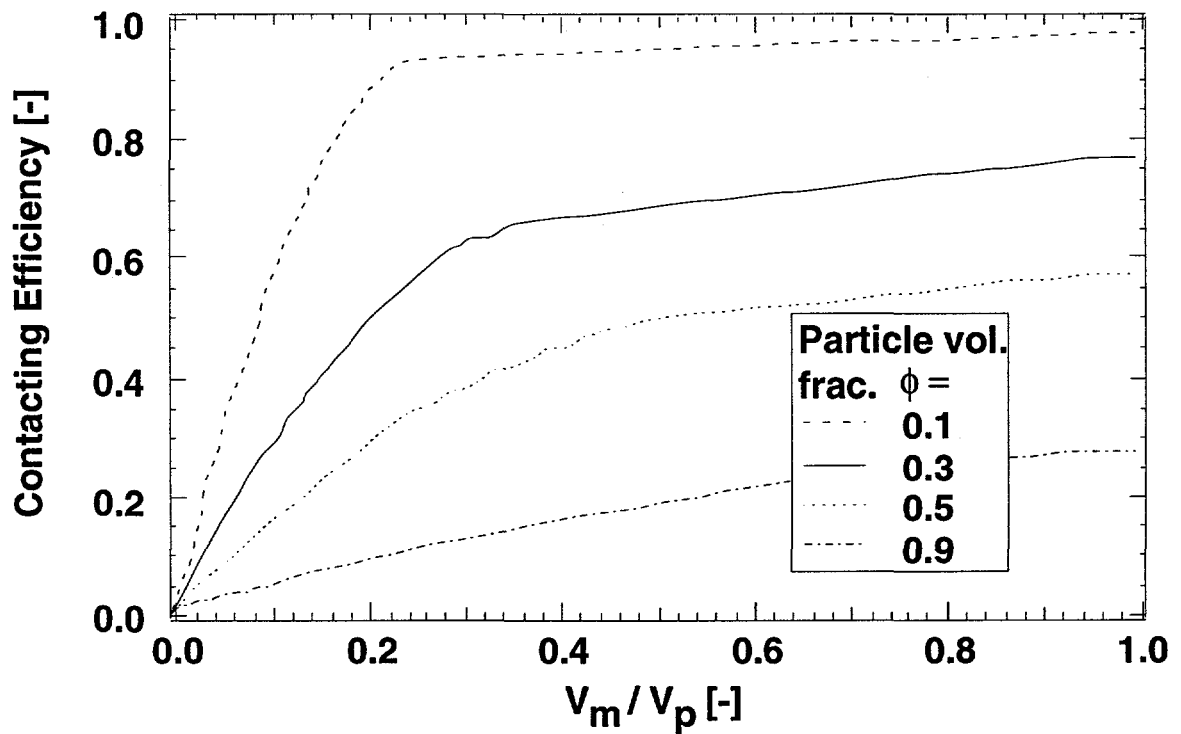
Figure 2.12 Quantitative dependence of contacting efficiency on relative proportions of molten on condensate volume to particulate volume.
